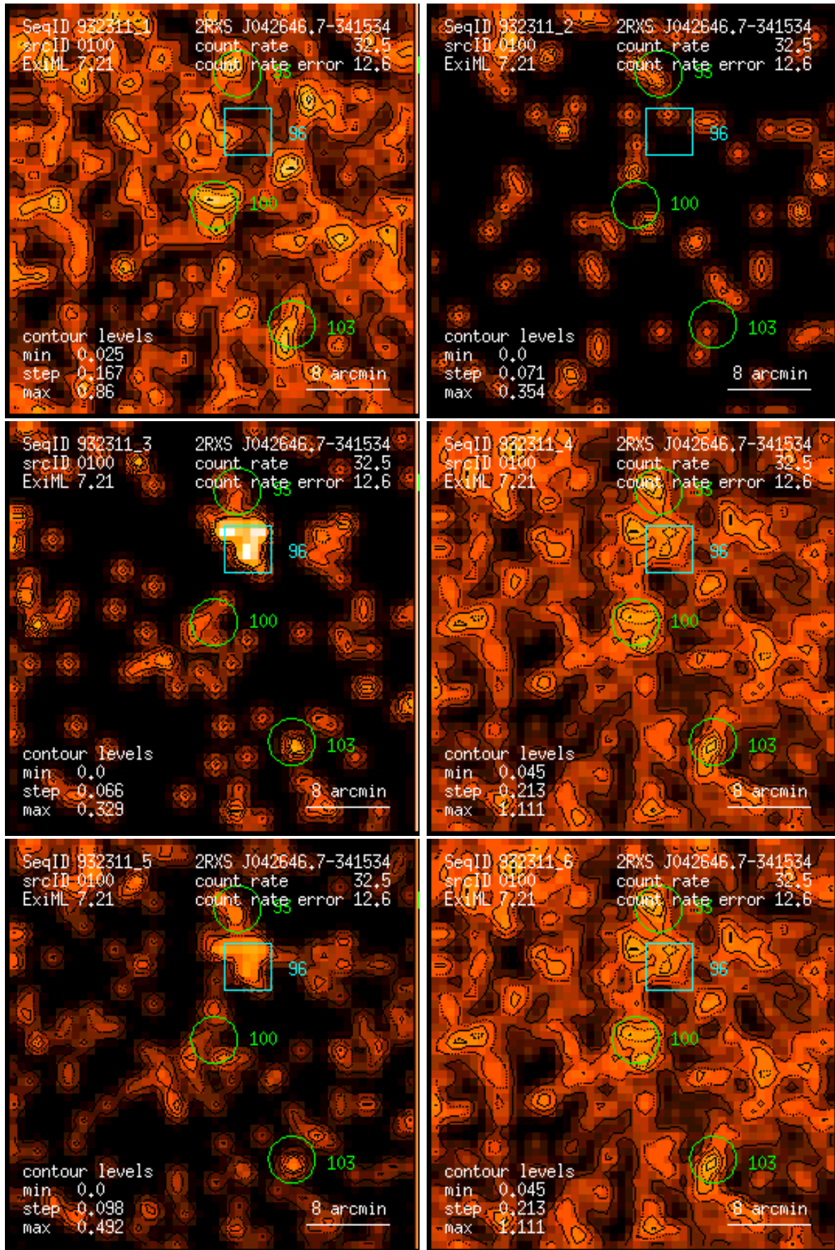
Figure 100: RASS 932311: detection 0100: band rate images, Gaussian filter: (1) PSPC channels 11 – 41, (2) 52 – 90, (3) 91 – 201, (4) 11 – 235, (5) 52 – 201, (6) 11 – 201. Broad band rates in counts/ks. Band rate contour levels in counts/ks/arcmin 2 .
