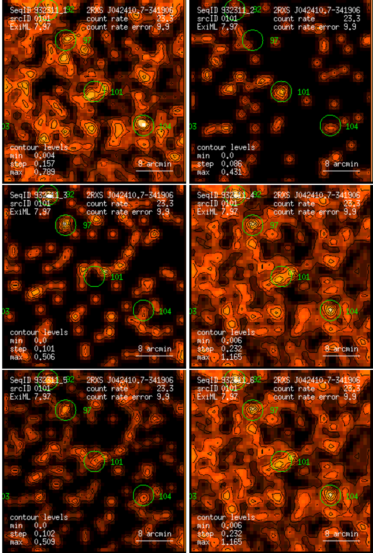
Figure 101: RASS 932311: detection 0101: band rate images, Gaussian filter: (1) PSPC channels 11 – 41, (2) 52 – 90, (3) 91 – 201, (4) 11 – 235, (5) 52 – 201, (6) 11 – 201. Broad band rates in counts/ks. Band rate contour levels in counts/ks/arcmin 2 .
