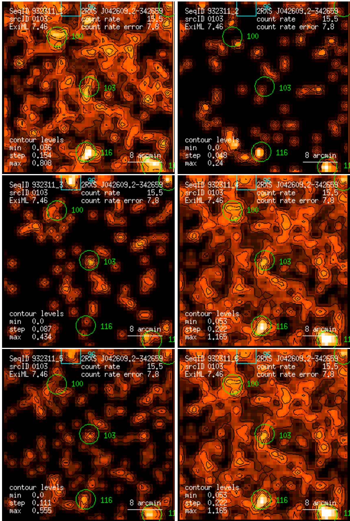
Figure 103: RASS 932311: detection 0103: band rate images, Gaussian filter: (1) PSPC channels 11 – 41, (2) 52 – 90, (3) 91 – 201, (4) 11 – 235, (5) 52 – 201, (6) 11 – 201. Broad band rates in counts/ks. Band rate contour levels in counts/ks/arcmin 2 .
