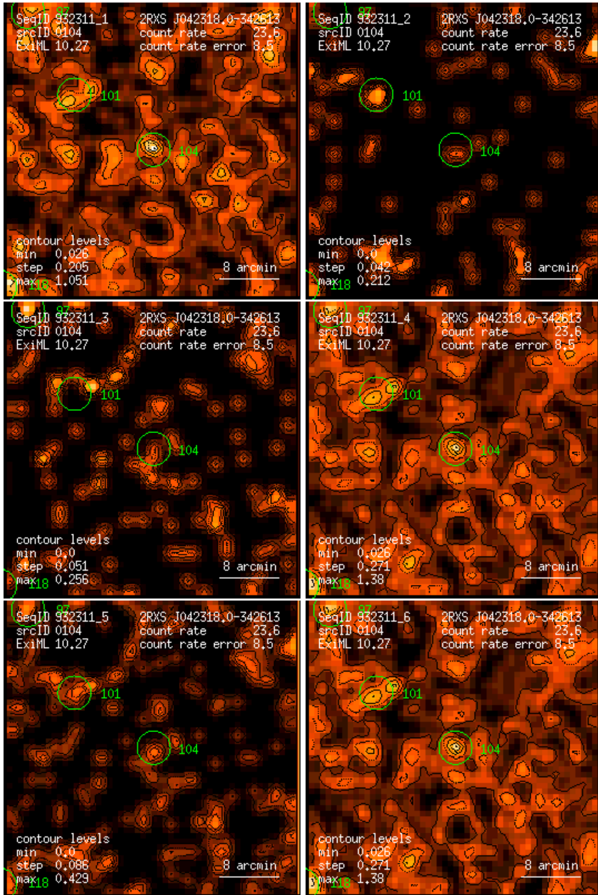
Figure 104: RASS 932311: detection 0104: band rate images, Gaussian filter: (1) PSPC channels 11 – 41, (2) 52 – 90, (3) 91 – 201, (4) 11 – 235, (5) 52 – 201, (6) 11 – 201. Broad band rates in counts/ks. Band rate contour levels in counts/ks/arcmin 2 .
