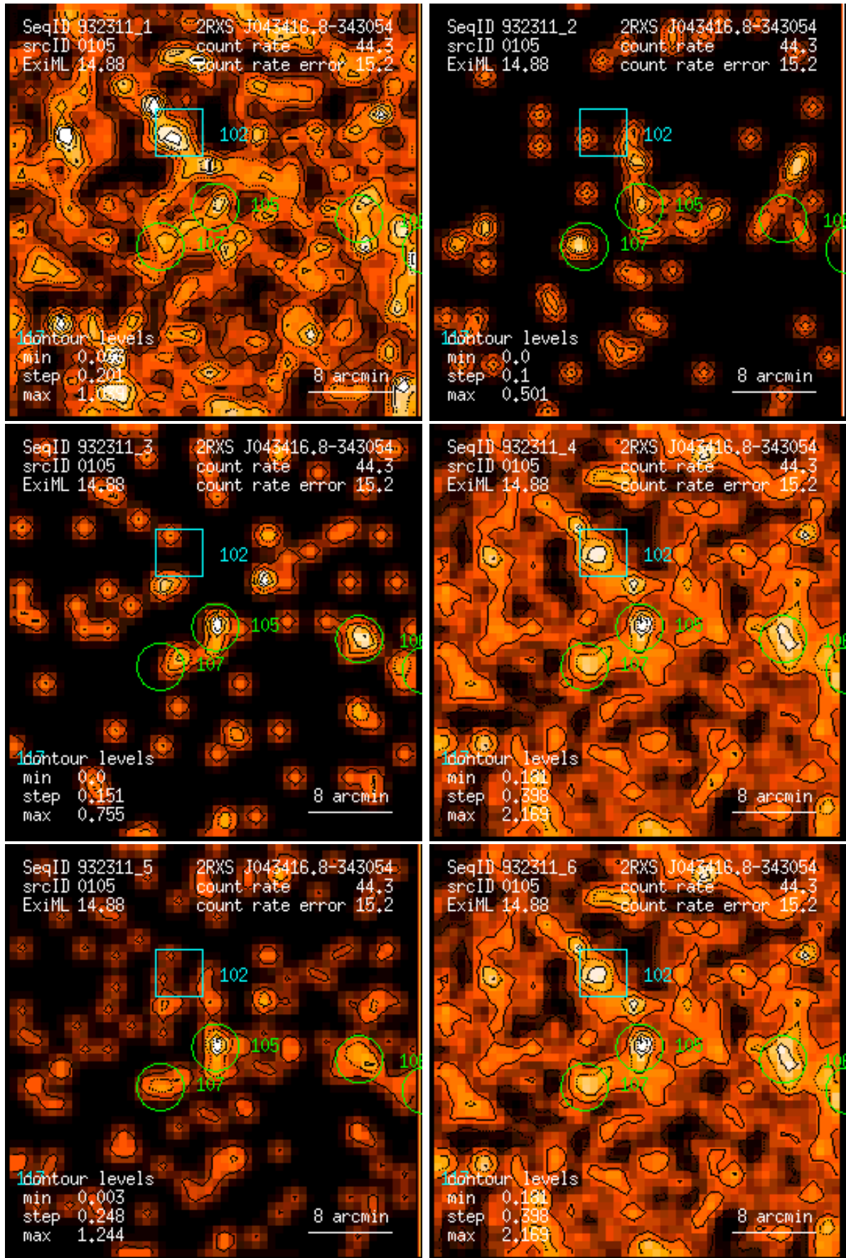
Figure 105: RASS 932311: detection 0105: band rate images, Gaussian filter: (1) PSPC channels 11 – 41, (2) 52 – 90, (3) 91 – 201, (4) 11 – 235, (5) 52 – 201, (6) 11 – 201. Broad band rates in counts/ks. Band rate contour levels in counts/ks/arcmin 2 .
