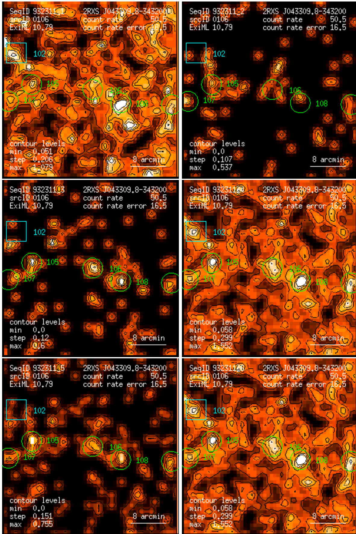
Figure 106: RASS 932311: detection 0106: band rate images, Gaussian filter: (1) PSPC channels 11 – 41, (2) 52 – 90, (3) 91 – 201, (4) 11 – 235, (5) 52 – 201, (6) 11 – 201. Broad band rates in counts/ks. Band rate contour levels in counts/ks/arcmin 2 .
