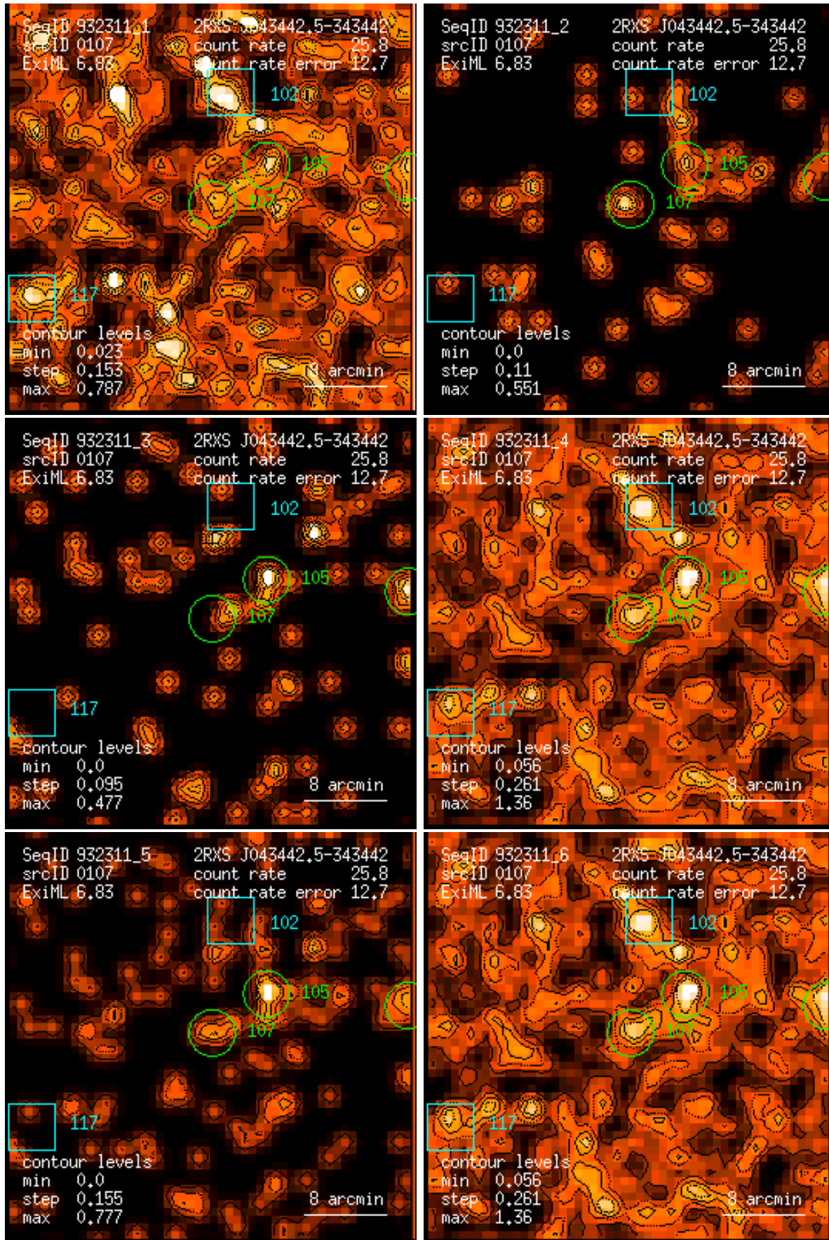
Figure 107: RASS 932311: detection 0107: band rate images, Gaussian filter: (1) PSPC channels 11 – 41, (2) 52 – 90, (3) 91 – 201, (4) 11 – 235, (5) 52 – 201, (6) 11 – 201. Broad band rates in counts/ks. Band rate contour levels in counts/ks/arcmin 2 .
