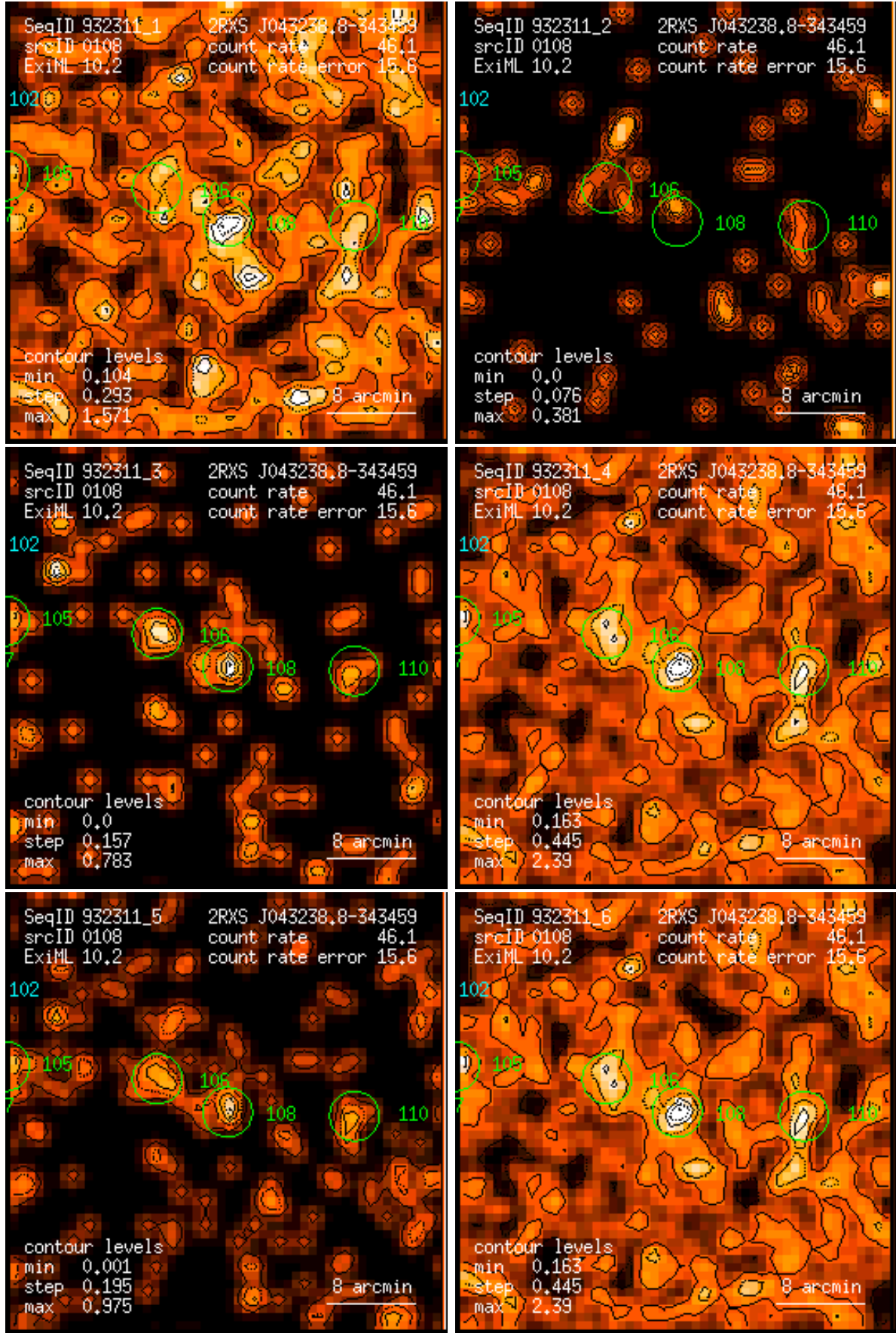
Figure 108: RASS 932311: detection 0108: band rate images, Gaussian filter: (1) PSPC channels 11 – 41, (2) 52 – 90, (3) 91 – 201, (4) 11 – 235, (5) 52 – 201, (6) 11 – 201. Broad band rates in counts/ks. Band rate contour levels in counts/ks/arcmin 2 .
