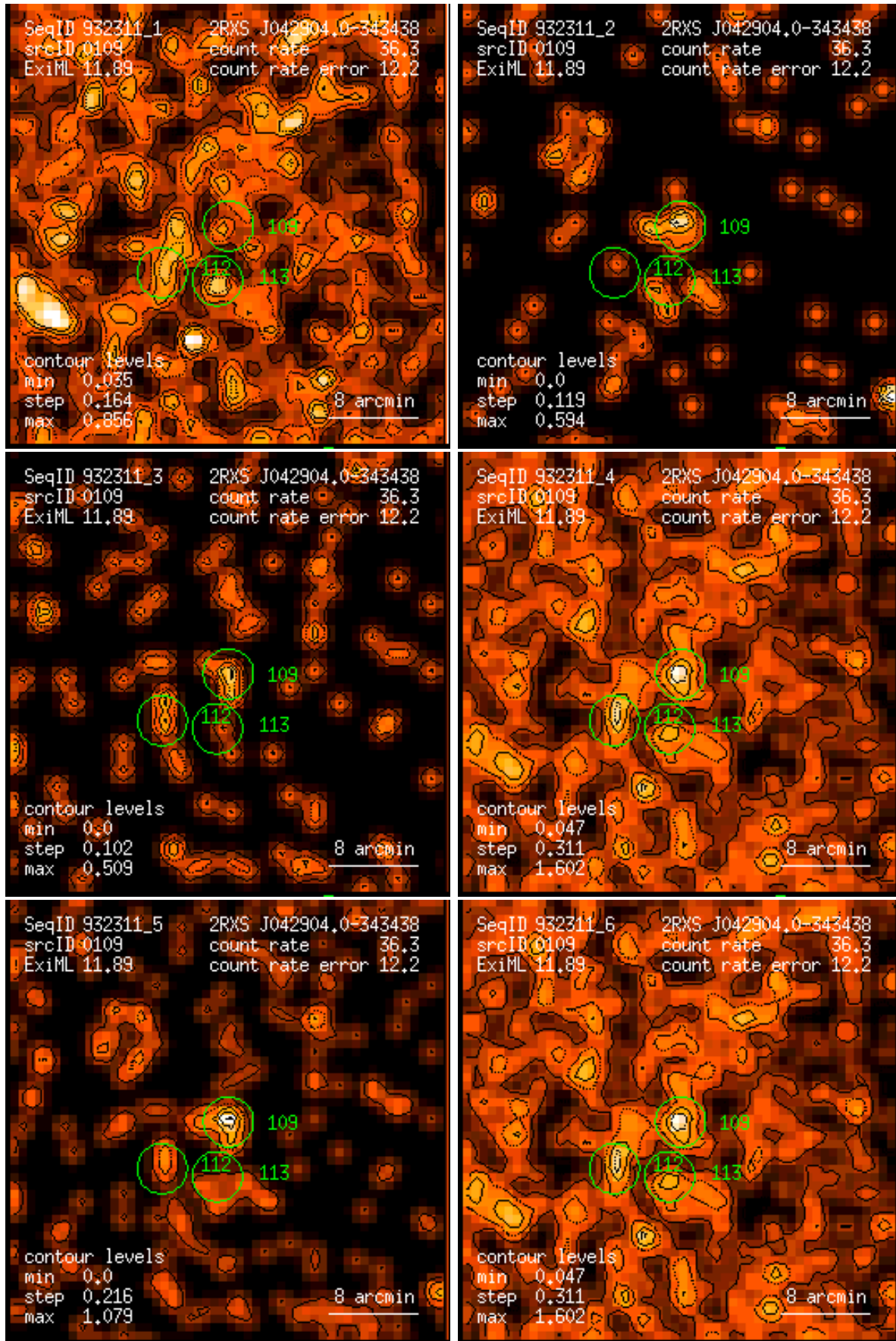
Figure 109: RASS 932311: detection 0109: band rate images, Gaussian filter: (1) PSPC channels 11 – 41, (2) 52 – 90, (3) 91 – 201, (4) 11 – 235, (5) 52 – 201, (6) 11 – 201. Broad band rates in counts/ks. Band rate contour levels in counts/ks/arcmin 2 .
