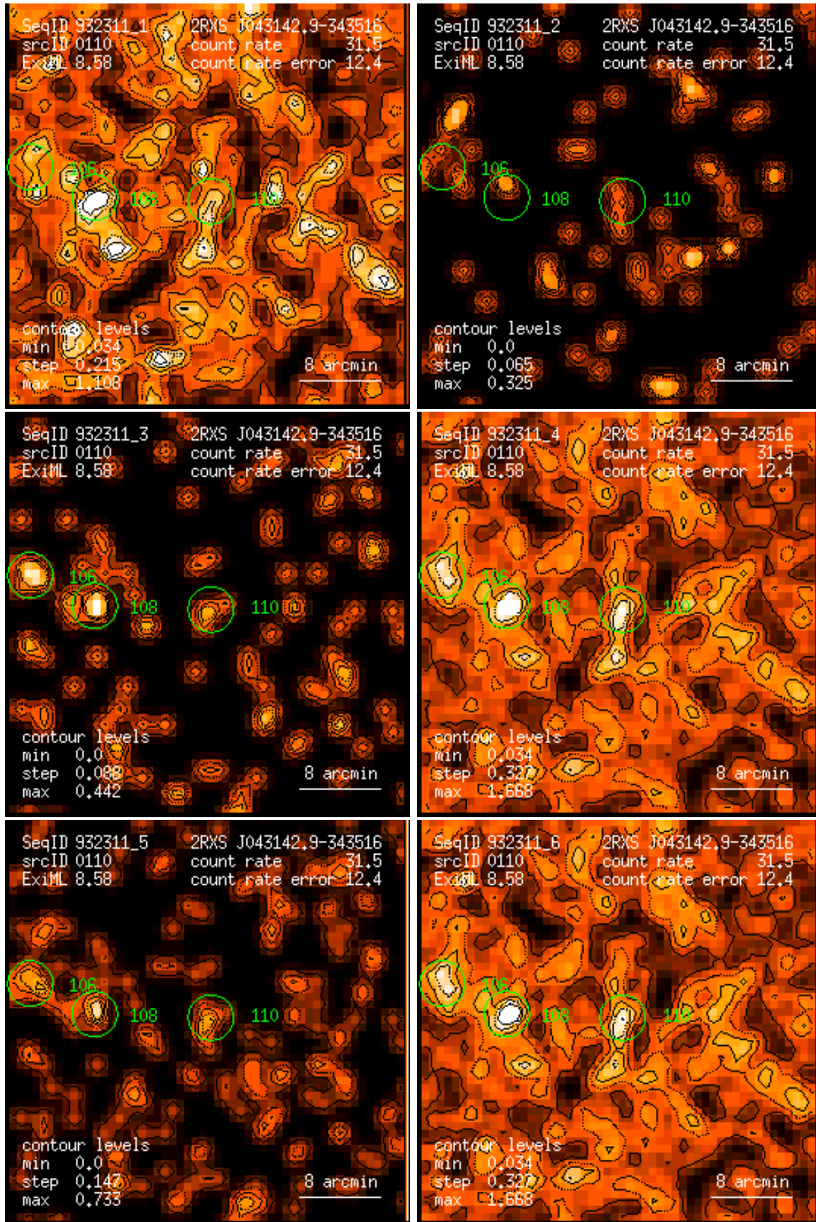
Figure 110: RASS 932311: detection 0110: band rate images, Gaussian filter: (1) PSPC channels 11 – 41, (2) 52 – 90, (3) 91 – 201, (4) 11 – 235, (5) 52 – 201, (6) 11 – 201. Broad band rates in counts/ks. Band rate contour levels in counts/ks/arcmin 2 .
