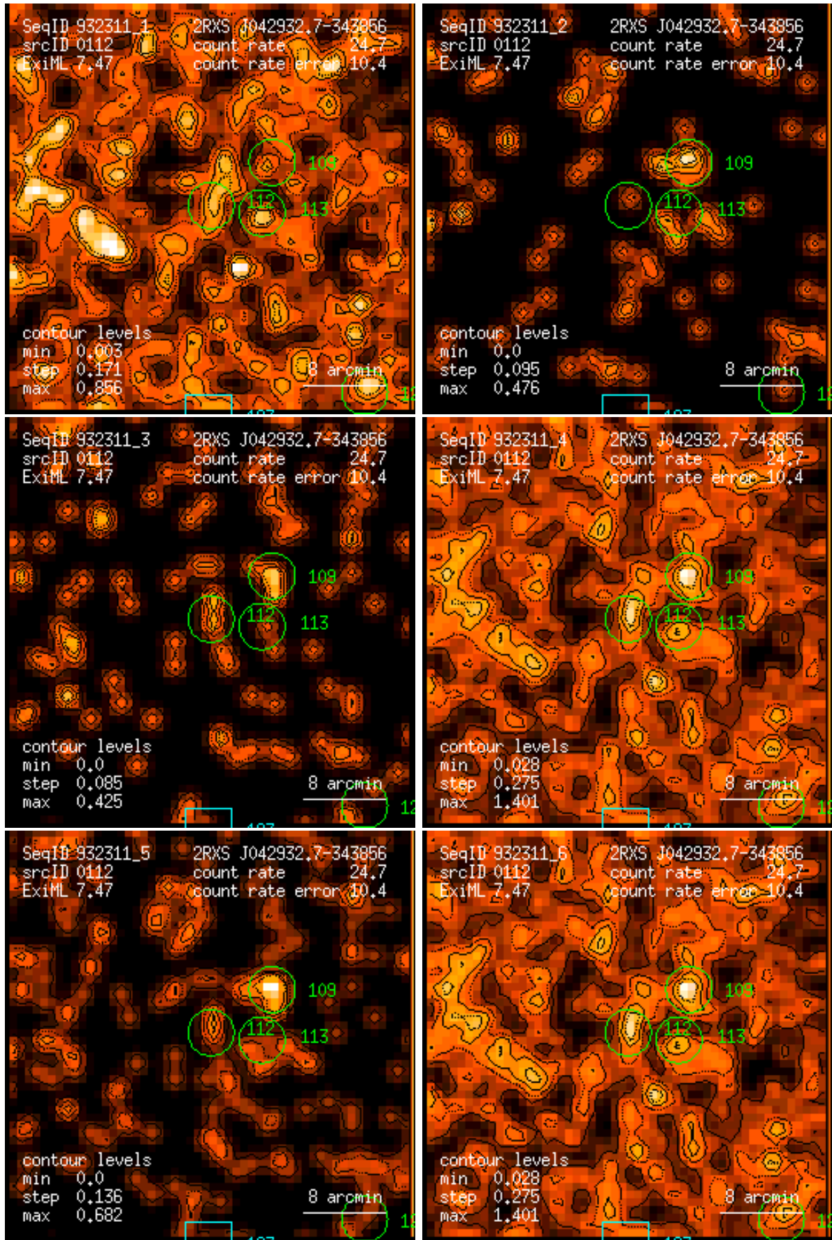
Figure 112: RASS 932311: detection 0112: band rate images, Gaussian filter: (1) PSPC channels 11 – 41, (2) 52 – 90, (3) 91 – 201, (4) 11 – 235, (5) 52 – 201, (6) 11 – 201. Broad band rates in counts/ks. Band rate contour levels in counts/ks/arcmin 2 .
