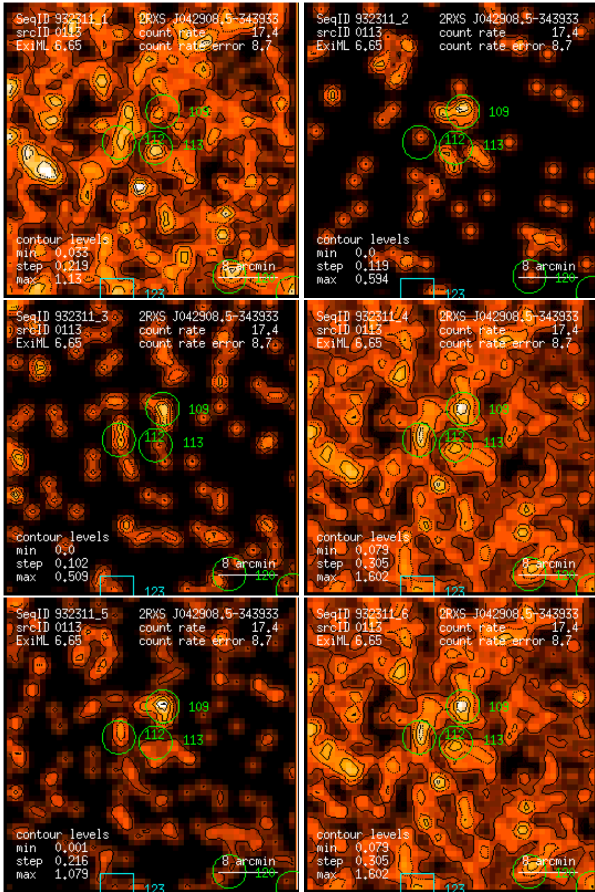
Figure 113: RASS 932311: detection 0113: band rate images, Gaussian filter: (1) PSPC channels 11 – 41, (2) 52 – 90, (3) 91 – 201, (4) 11 – 235, (5) 52 – 201, (6) 11 – 201. Broad band rates in counts/ks. Band rate contour levels in counts/ks/arcmin 2 .
