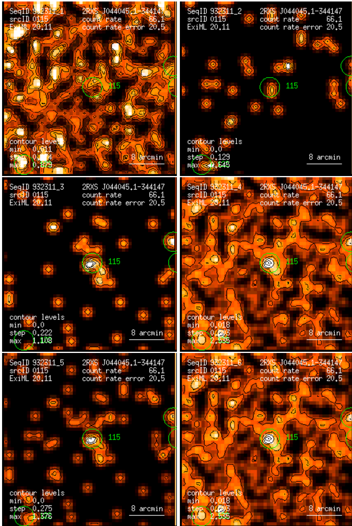
Figure 115: RASS 932311: detection 0115: band rate images, Gaussian filter: (1) PSPC channels 11 – 41, (2) 52 – 90, (3) 91 – 201, (4) 11 – 235, (5) 52 – 201, (6) 11 – 201. Broad band rates in counts/ks. Band rate contour levels in counts/ks/arcmin 2 .
