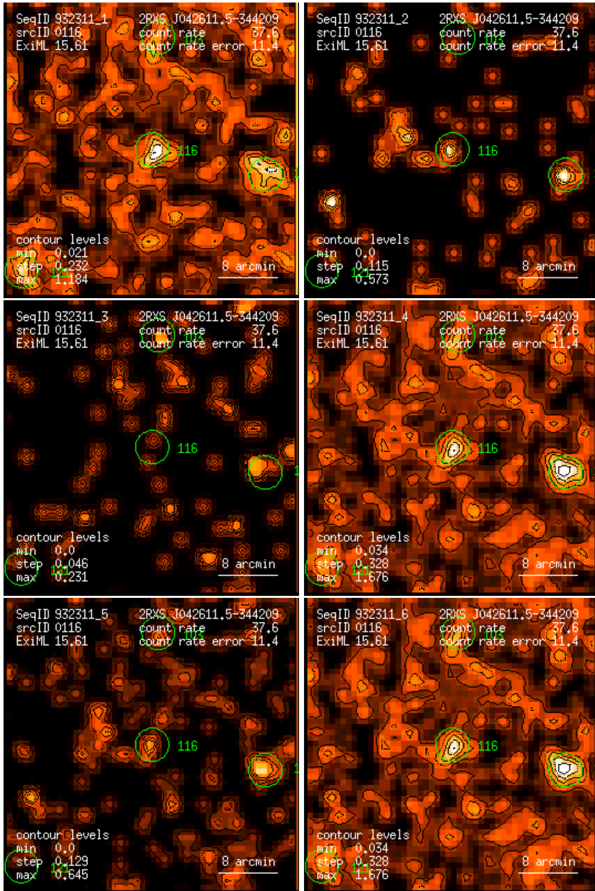
Figure 116: RASS 932311: detection 0116: band rate images, Gaussian filter: (1) PSPC channels 11 – 41, (2) 52 – 90, (3) 91 – 201, (4) 11 – 235, (5) 52 – 201, (6) 11 – 201. Broad band rates in counts/ks. Band rate contour levels in counts/ks/arcmin 2 .
