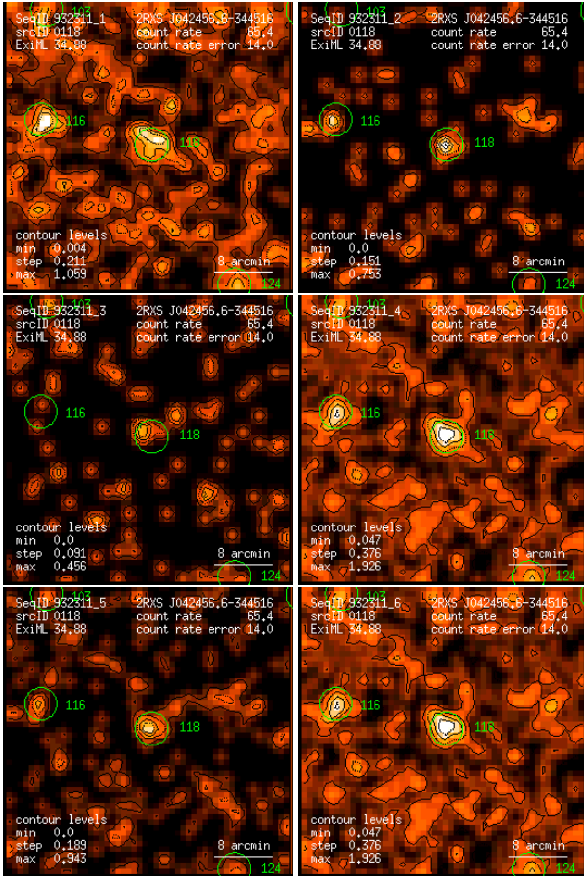
Figure 118: RASS 932311: detection 0118: band rate images, Gaussian filter: (1) PSPPC channels 11 – 41, (2) 52 – 90, (3) 91 – 201, (4) 11 – 235, (5) 52 – 201, (6) 11 – 201. Broad band rates in counts/ks. Band rate contour levels in counts/ks/arcmin 2 .
