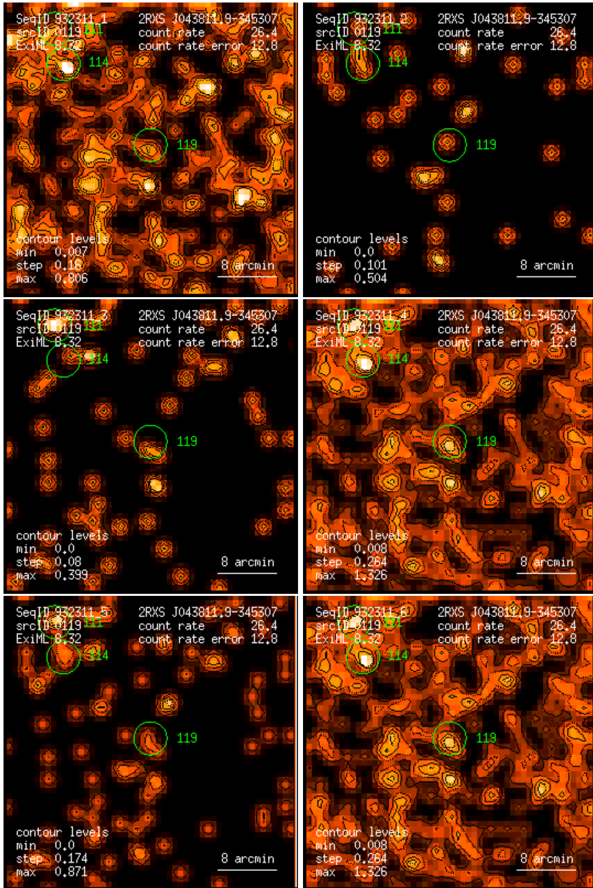
Figure 119: RASS 932311: detection 0119: band rate images, Gaussian filter: (1) PSPC channels 11 – 41, (2) 52 – 90, (3) 91 – 201, (4) 11 – 235, (5) 52 – 201, (6) 11 – 201. Broad band rates in counts/ks. Band rate contour levels in counts/ks/arcmin 2 .
