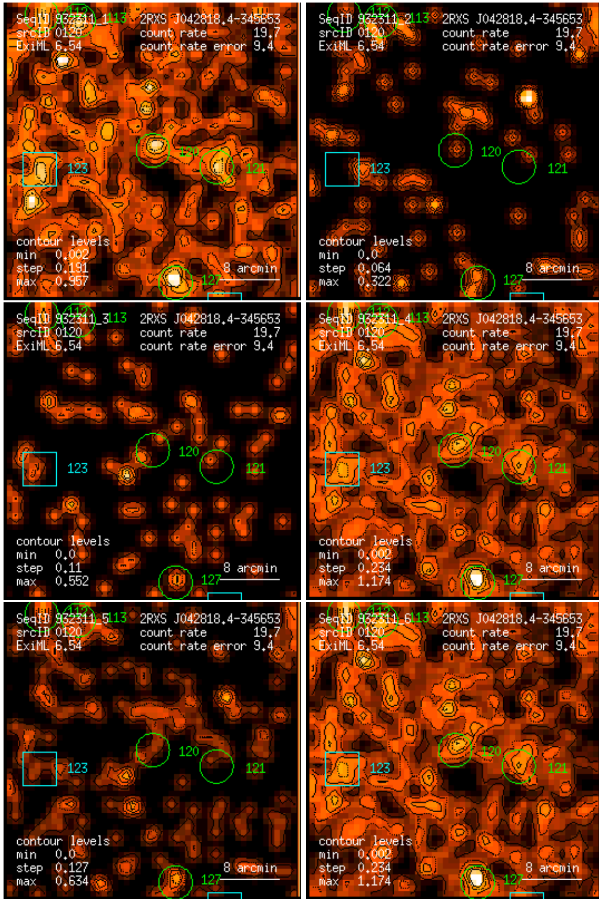
Figure 120: RASS 932311: detection 0120: band rate images, Gaussian filter: (1) PSPC channels 11 – 41, (2) 52 – 90, (3) 91 – 201, (4) 11 – 235, (5) 52 – 201, (6) 11 – 201. Broad band rates in counts/ks. Band rate contour levels in counts/ks/arcmin 2 .
