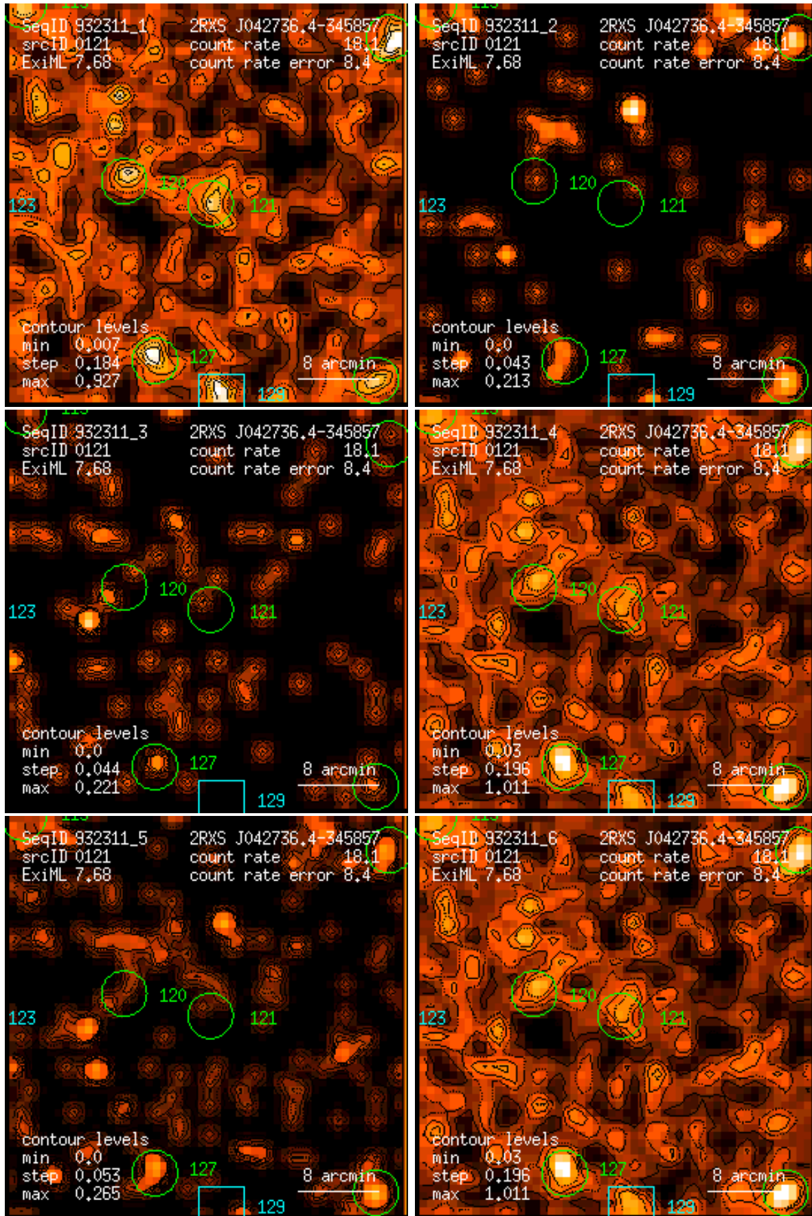
Figure 121: RASS 932311: detection 0121: band rate images, Gaussian filter: (1) PSPC channels 11 – 41, (2) 52 – 90, (3) 91 – 201, (4) 11 – 235, (5) 52 – 201, (6) 11 – 201. Broad band rates in counts/ks. Band rate contour levels in counts/ks/arcmin 2 .
