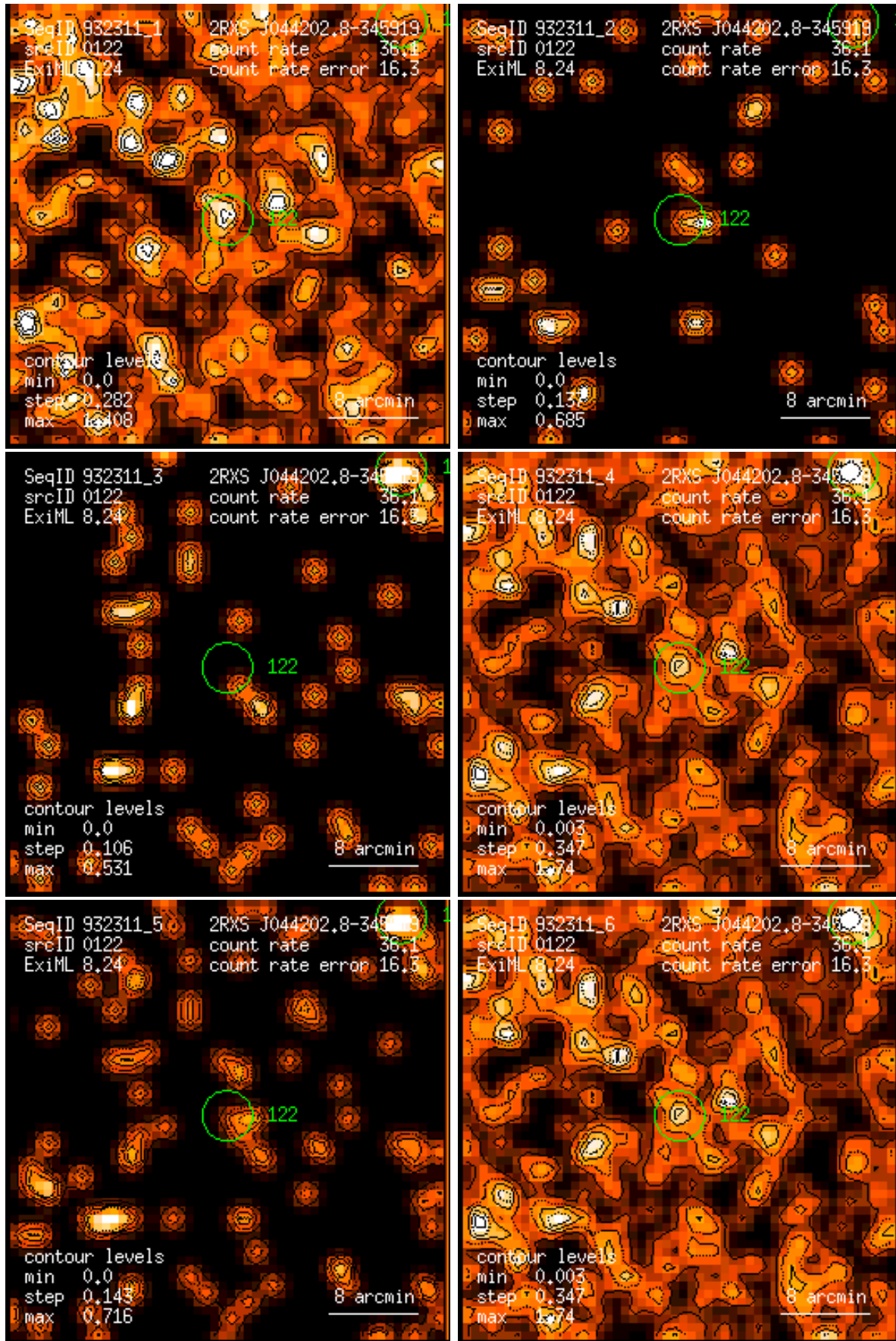
Figure 122: RASS 932311: detection 0122: band rate images, Gaussian filter: (1) PSPC channels 11 – 41, (2) 52 – 90, (3) 91 – 201, (4) 11 – 235, (5) 52 – 201, (6) 11 – 201. Broad band rates in counts/ks. Band rate contour levels in counts/ks/arcmin 2 .
