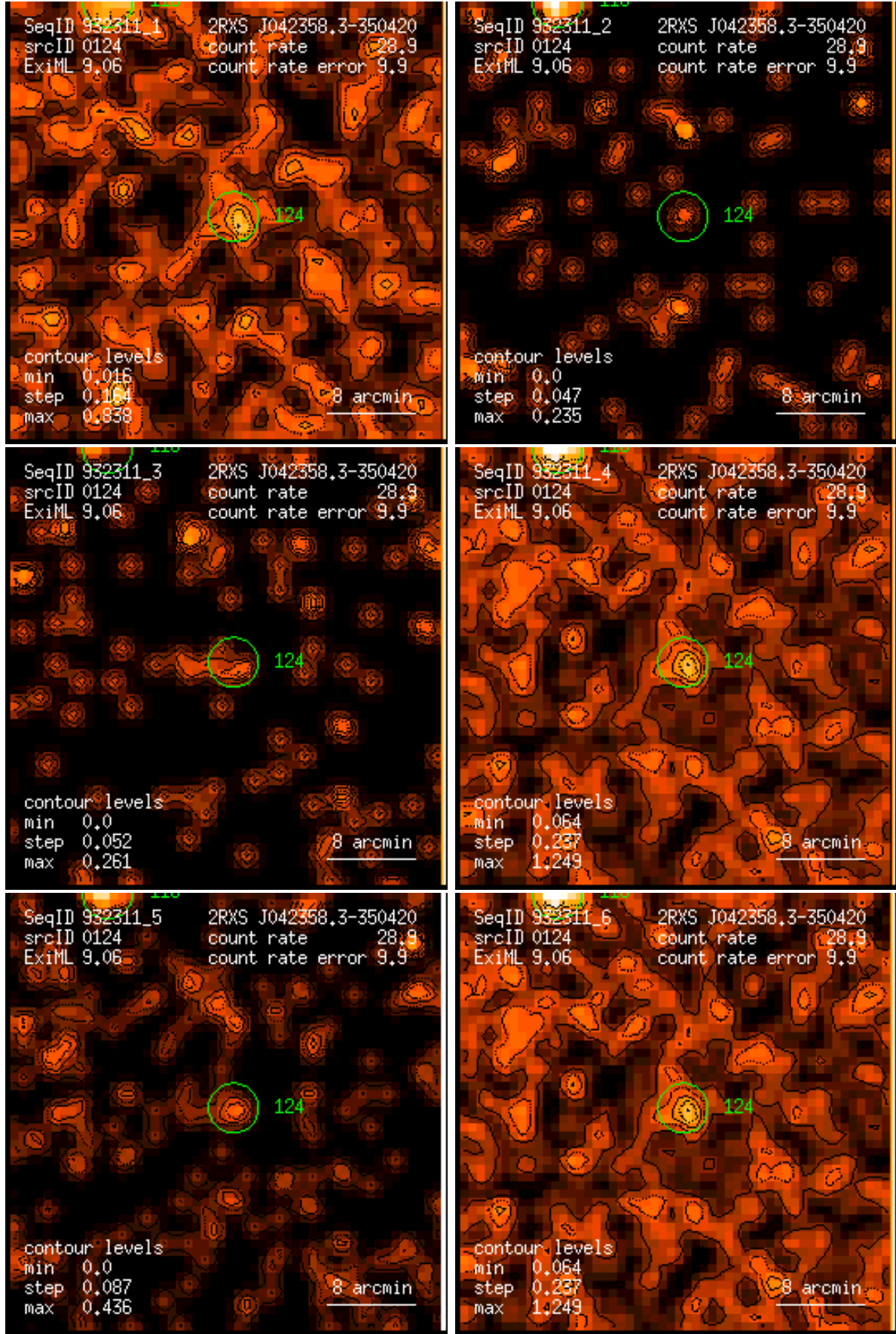
Figure 124: RASS 932311: detection 0124: band rate images, Gaussian filter: (1) PSPC channels 11 – 41, (2) 52 – 90, (3) 91 – 201, (4) 11 – 235, (5) 52 – 201, (6) 11 – 201. Broad band rates in counts/ks. Band rate contour levels in counts/ks/arcmin 2 .
