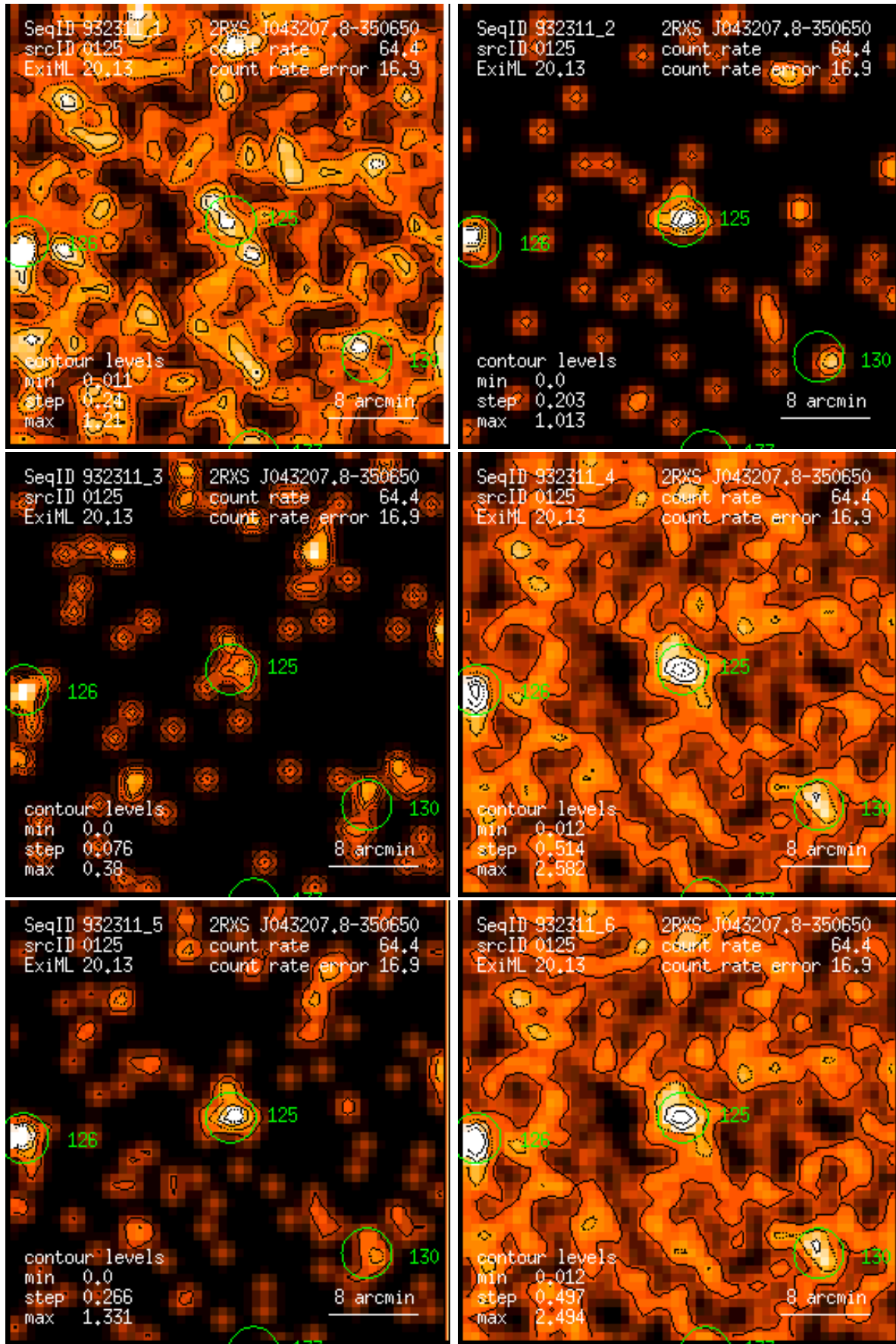
Figure 125: RASS 932311: detection 0125: band rate images, Gaussian filter: (1) PSPC channels 11 – 41, (2) 52 – 90, (3) 91 – 201, (4) 11 – 235, (5) 52 – 201, (6) 11 – 201. Broad band rates in counts/ks. Band rate contour levels in counts/ks/arcmin 2 .
