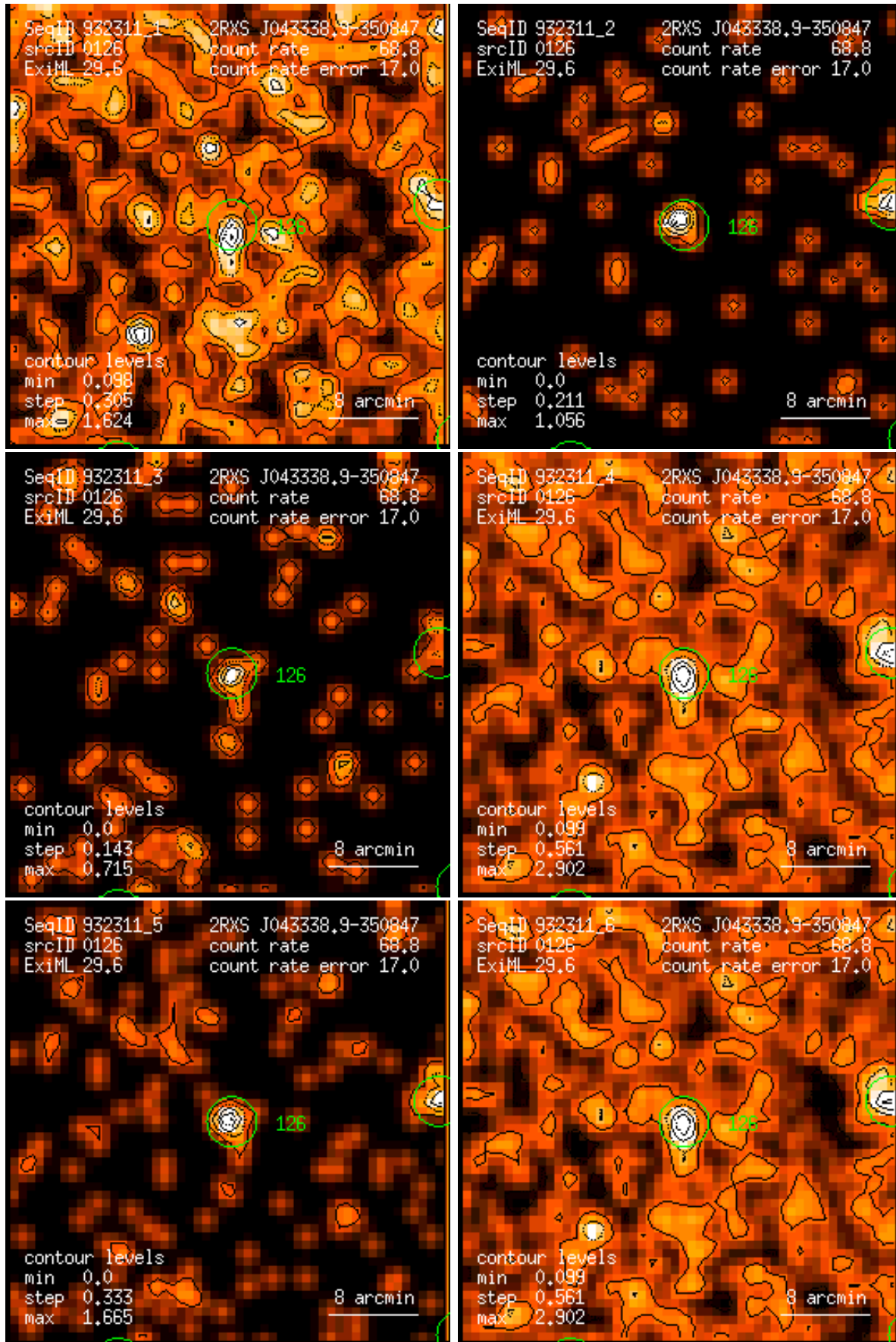
Figure 126: RASS 932311: detection 0126: band rate images, Gaussian filter: (1) PSPC channels 11 – 41, (2) 52 – 90, (3) 91 – 201, (4) 11 – 235, (5) 52 – 201, (6) 11 – 201. Broad band rates in counts/ks. Band rate contour levels in counts/ks/arcmin 2 .
