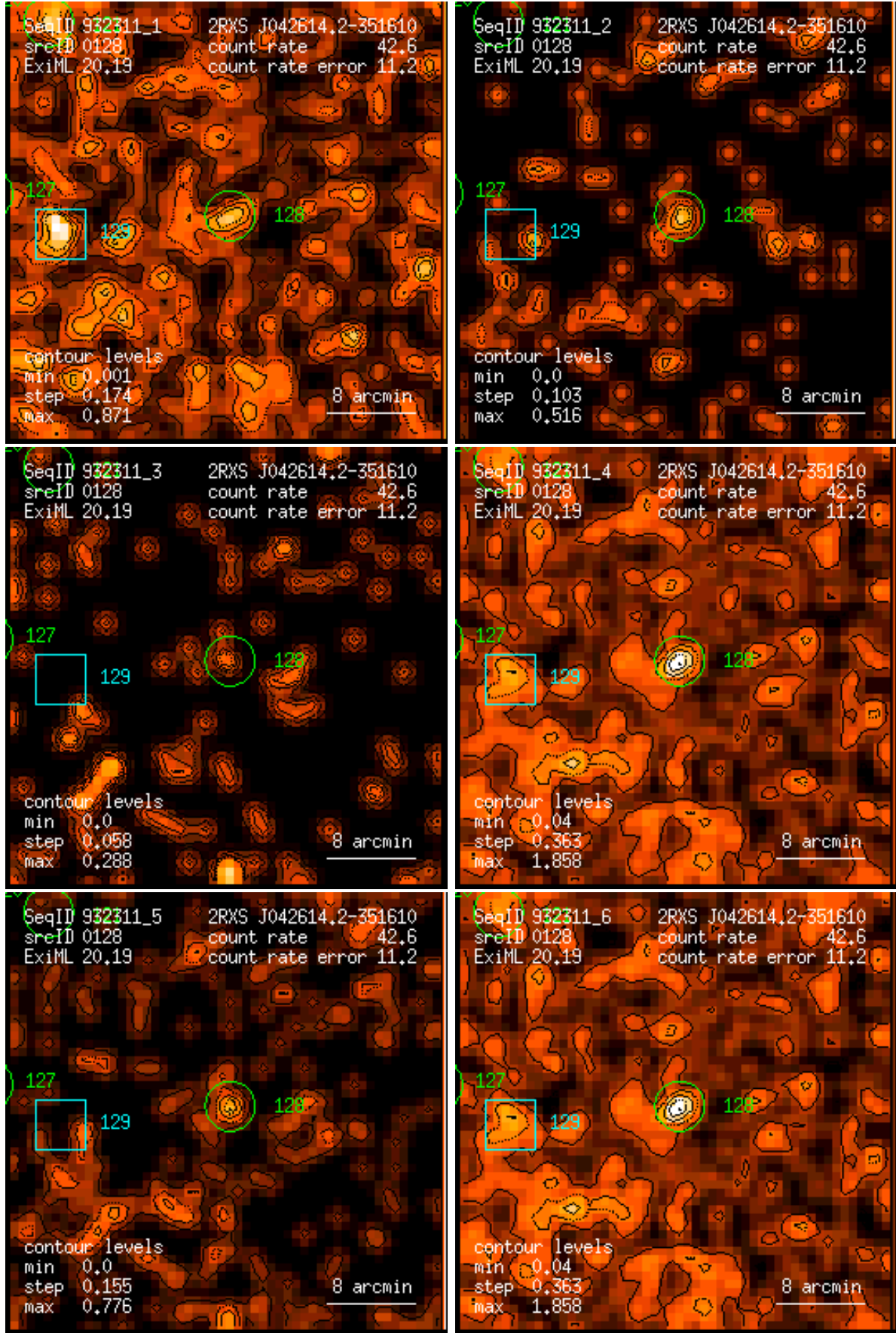
Figure 128: RASS 932311: detection 0128: band rate images, Gaussian filter: (1) PSPC channels 11 – 41, (2) 52 – 90, (3) 91 – 201, (4) 11 – 235, (5) 52 – 201, (6) 11 – 201. Broad band rates in counts/ks. Band rate contour levels in counts/ks/arcmin 2 .
