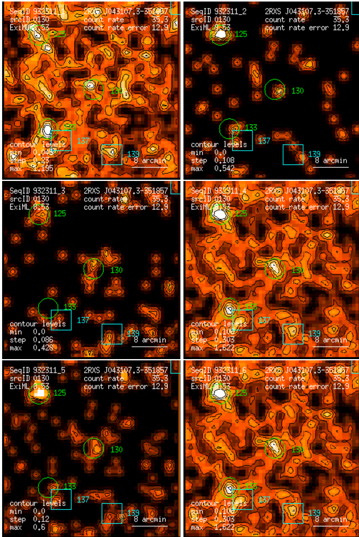
Figure 130: RASS 932311: detection 0130: band rate images, Gaussian filter: (1) PSPC channels 11 – 41, (2) 52 – 90, (3) 91 – 201, (4) 11 – 235, (5) 52 – 201, (6) 11 – 201. Broad band rates in counts/ks. Band rate contour levels in counts/ks/arcmin 2 .
