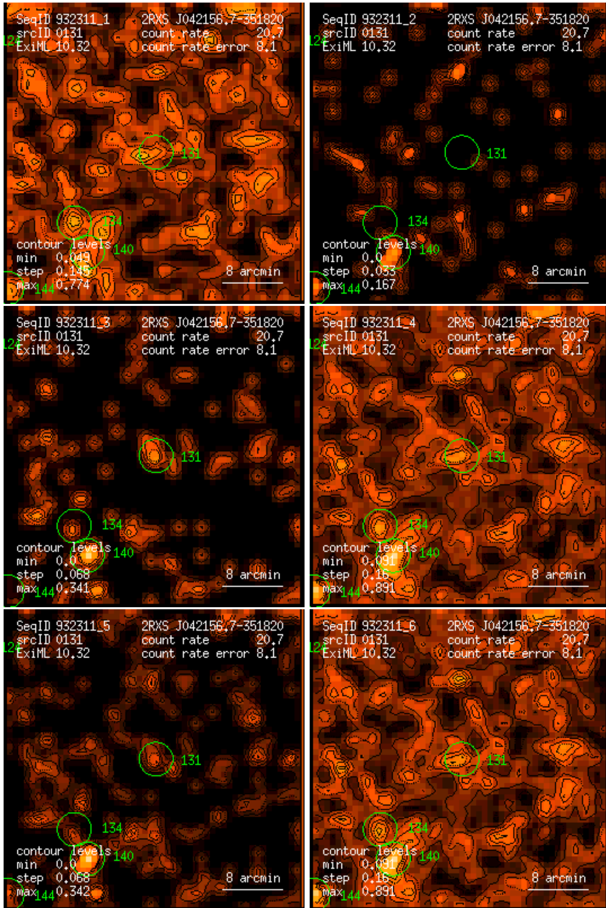
Figure 131: RASS 932311: detection 0131: band rate images, Gaussian filter: (1) PSPC channels 11 – 41, (2) 52 – 90, (3) 91 – 201, (4) 11 – 235, (5) 52 – 201, (6) 11 – 201. Broad band rates in counts/ks. Band rate contour levels in counts/ks/arcmin 2 .
