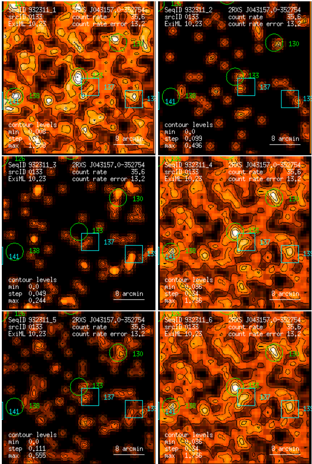
Figure 133: RASS 932311: detection 0133: band rate images, Gaussian filter: (1) PSPC channels 11 – 41, (2) 52 – 90, (3) 91 – 201, (4) 11 – 235, (5) 52 – 201, (6) 11 – 201. Broad band rates in counts/ks. Band rate contour levels in counts/ks/arcmin 2 .
