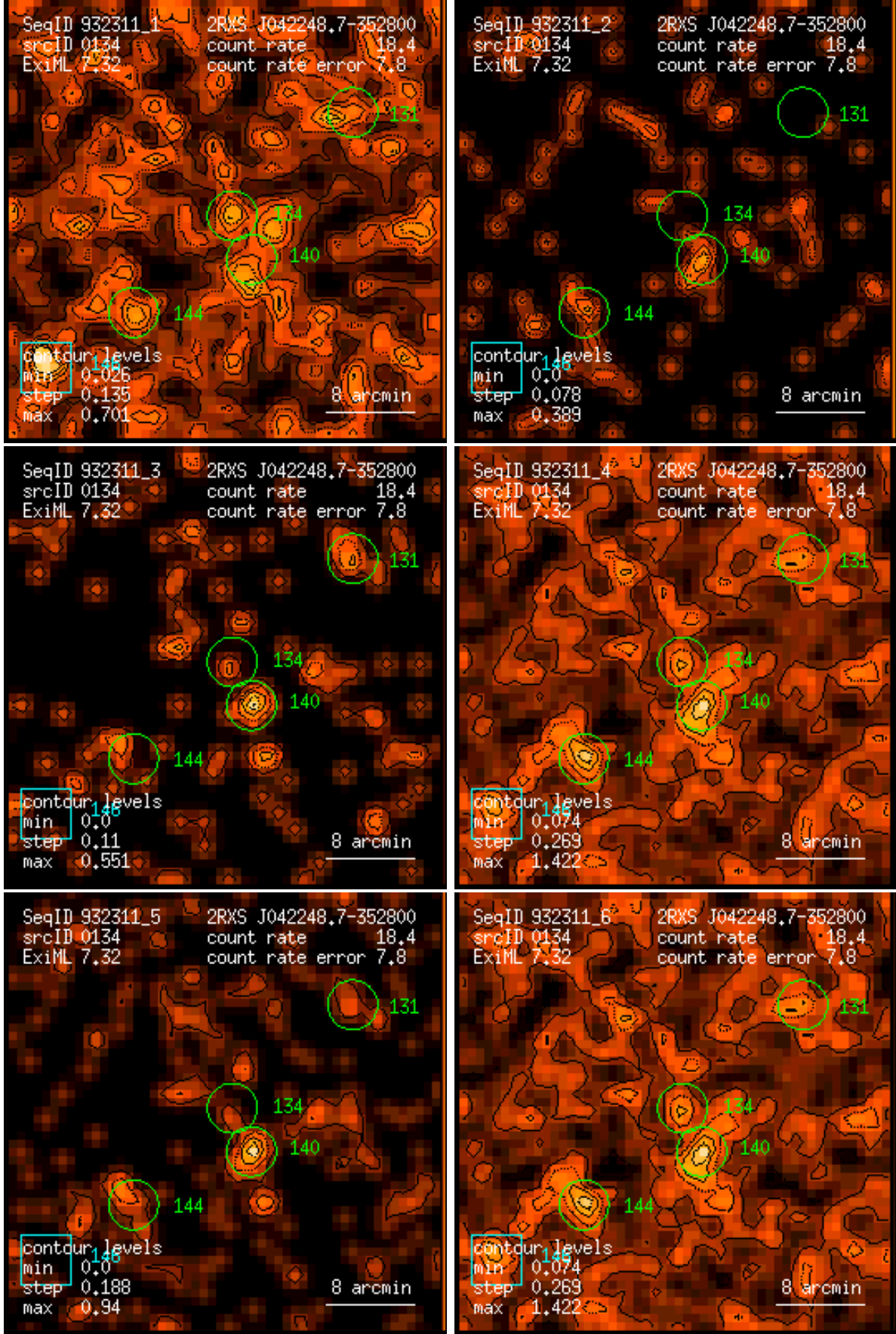
Figure 134: RASS 932311: detection 0134: band rate images, Gaussian filter: (1) PSPC channels 11 – 41, (2) 52 – 90, (3) 91 – 201, (4) 11 – 235, (5) 52 – 201, (6) 11 – 201. Broad band rates in counts/ks. Band rate contour levels in counts/ks/arcmin 2 .
