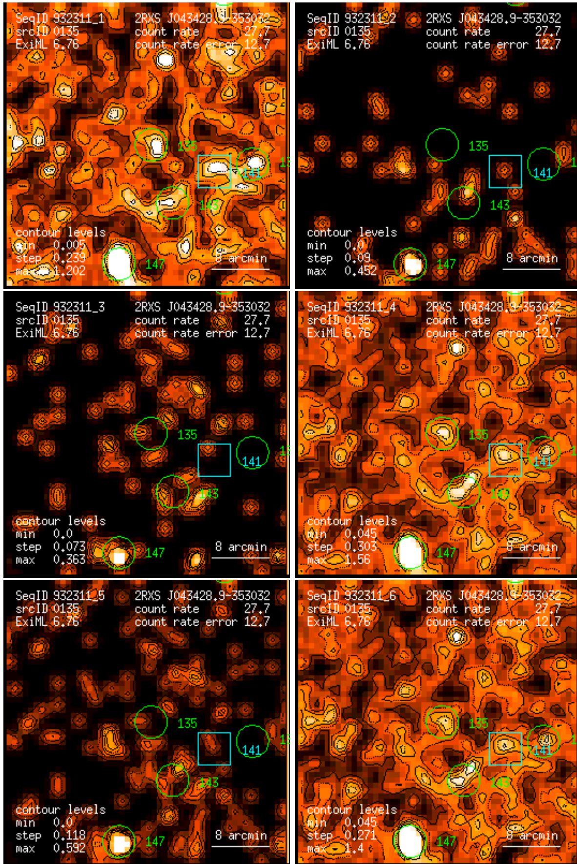
Figure 135: RASS 932311: detection 0135: band rate images, Gaussian filter: (1) PSPC channels 11 – 41, (2) 52 – 90, (3) 91 – 201, (4) 11 – 235, (5) 52 – 201, (6) 11 – 201. Broad band rates in counts/ks. Band rate contour levels in counts/ks/arcmin 2 .
