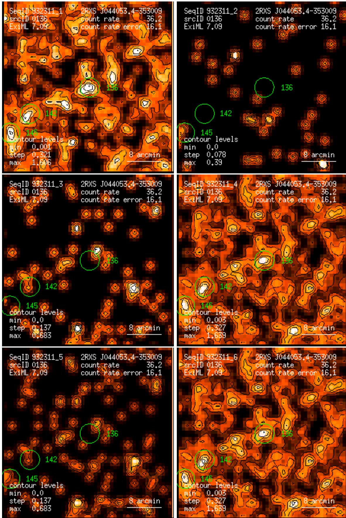
Figure 136: RASS 932311: detection 0136: band rate images, Gaussian filter: (1) PSPC channels 11 – 41, (2) 52 – 90, (3) 91 – 201, (4) 11 – 235, (5) 52 – 201, (6) 11 – 201. Broad band rates in counts/ks. Band rate contour levels in counts/ks/arcmin 2 .
