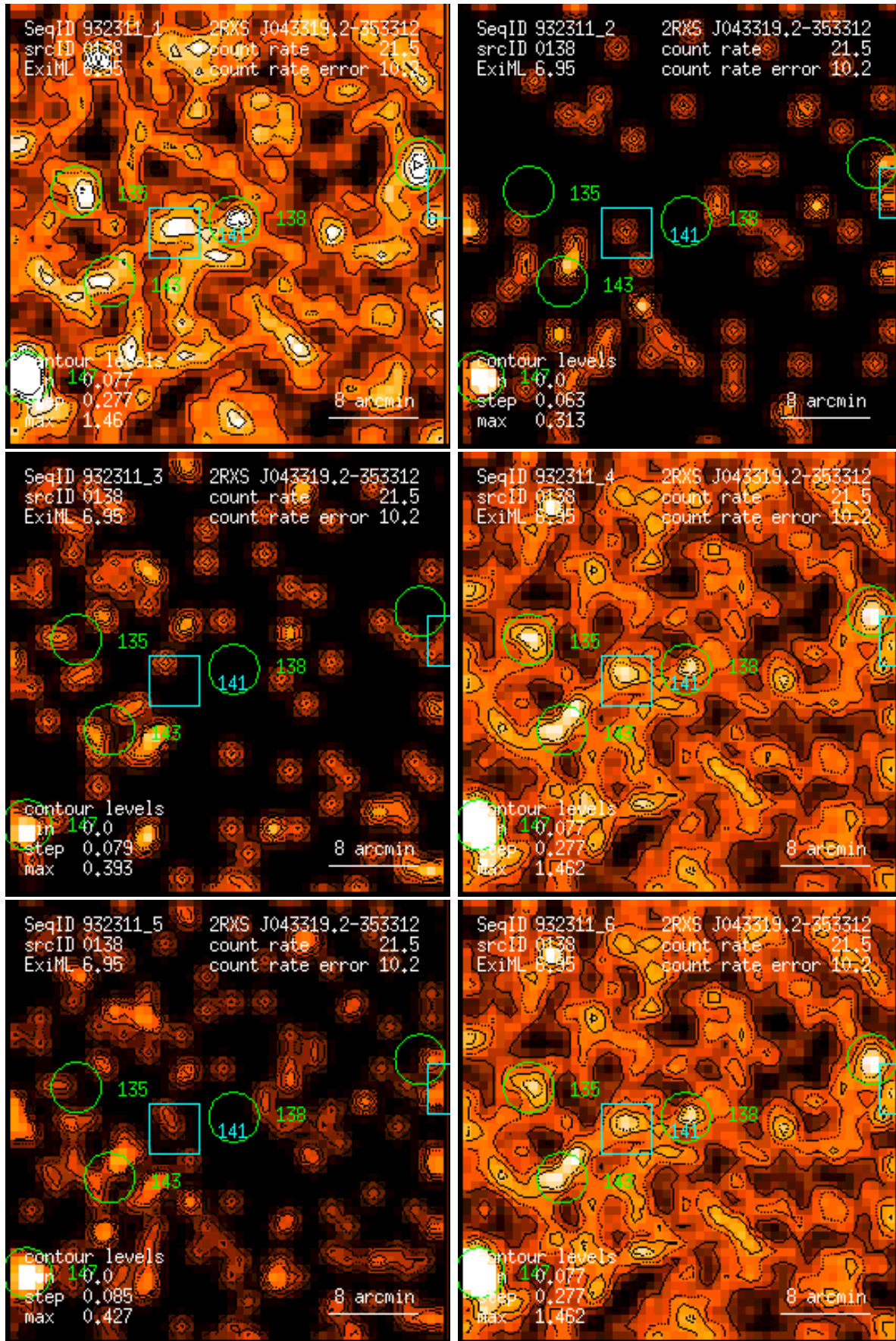
Figure 138: RASS 932311: detection 0138: band rate images, Gaussian filter: (1) PSPC channels 11 – 41, (2) 52 – 90, (3) 91 – 201, (4) 11 – 235, (5) 52 – 201, (6) 11 – 201. Broad band rates in counts/ks. Band rate contour levels in counts/ks/arcmin 2 .
