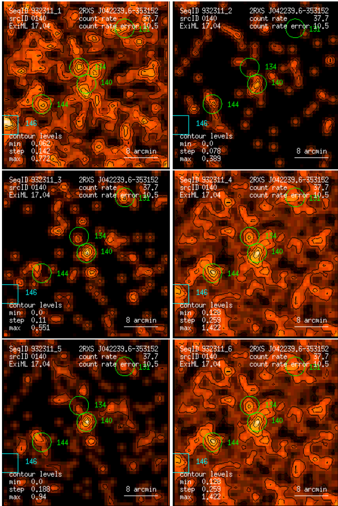
Figure 140: RASS 932311: detection 0140: band rate images, Gaussian filter: (1) PSPC channels 11 – 41, (2) 52 – 90, (3) 91 – 201, (4) 11 – 235, (5) 52 – 201, (6) 11 – 201. Broad band rates in counts/ks. Band rate contour levels in counts/ks/arcmin 2 .
