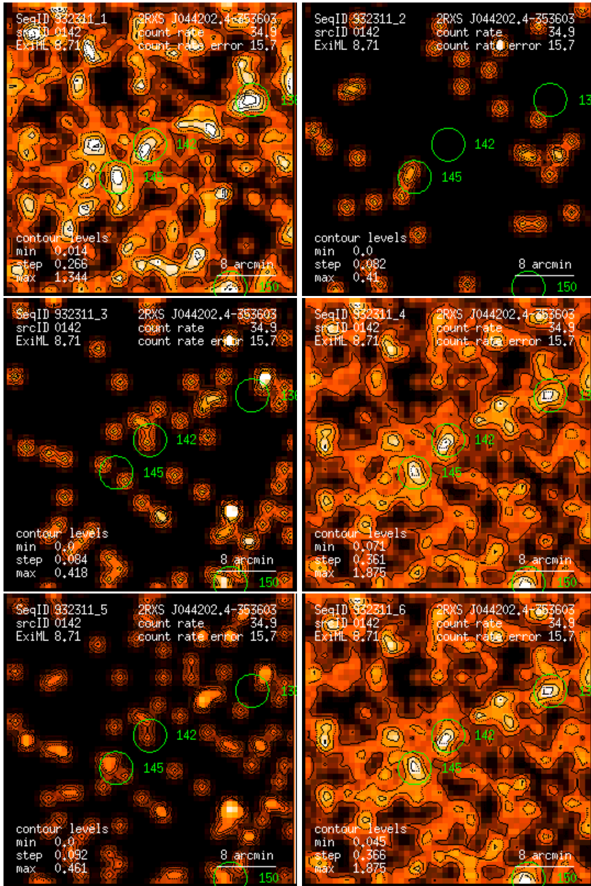
Figure 142: RASS 932311: detection 0142: band rate images, Gaussian filter: (1) PSPC channels 11 – 41, (2) 52 – 90, (3) 91 – 201, (4) 11 – 235, (5) 52 – 201, (6) 11 – 201. Broad band rates in counts/ks. Band rate contour levels in counts/ks/arcmin 2 .
