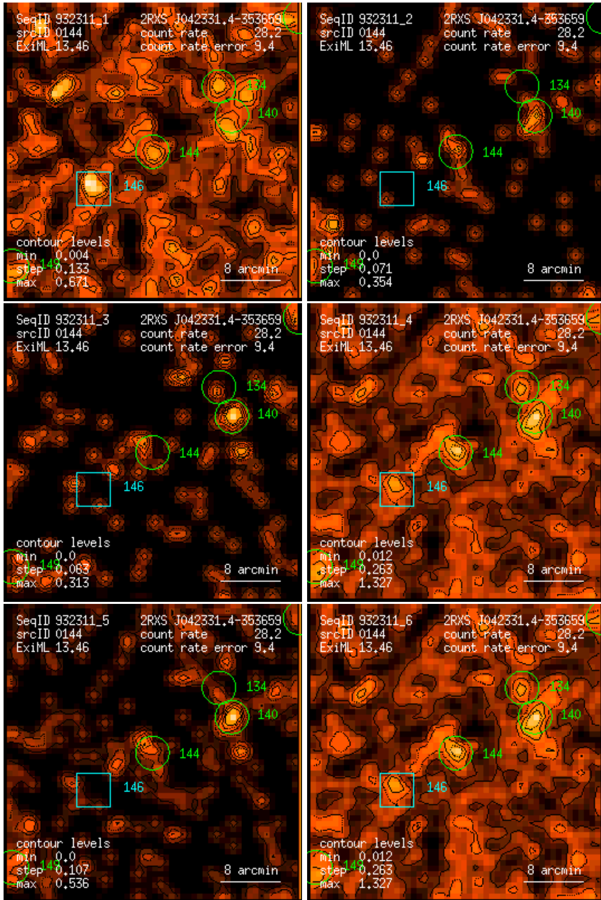
Figure 144: RASS 932311: detection 0144: band rate images, Gaussian filter: (1) PSPC channels 11 – 41, (2) 52 – 90, (3) 91 – 201, (4) 11 – 235, (5) 52 – 201, (6) 11 – 201. Broad band rates in counts/ks. Band rate contour levels in counts/ks/arcmin 2 .
