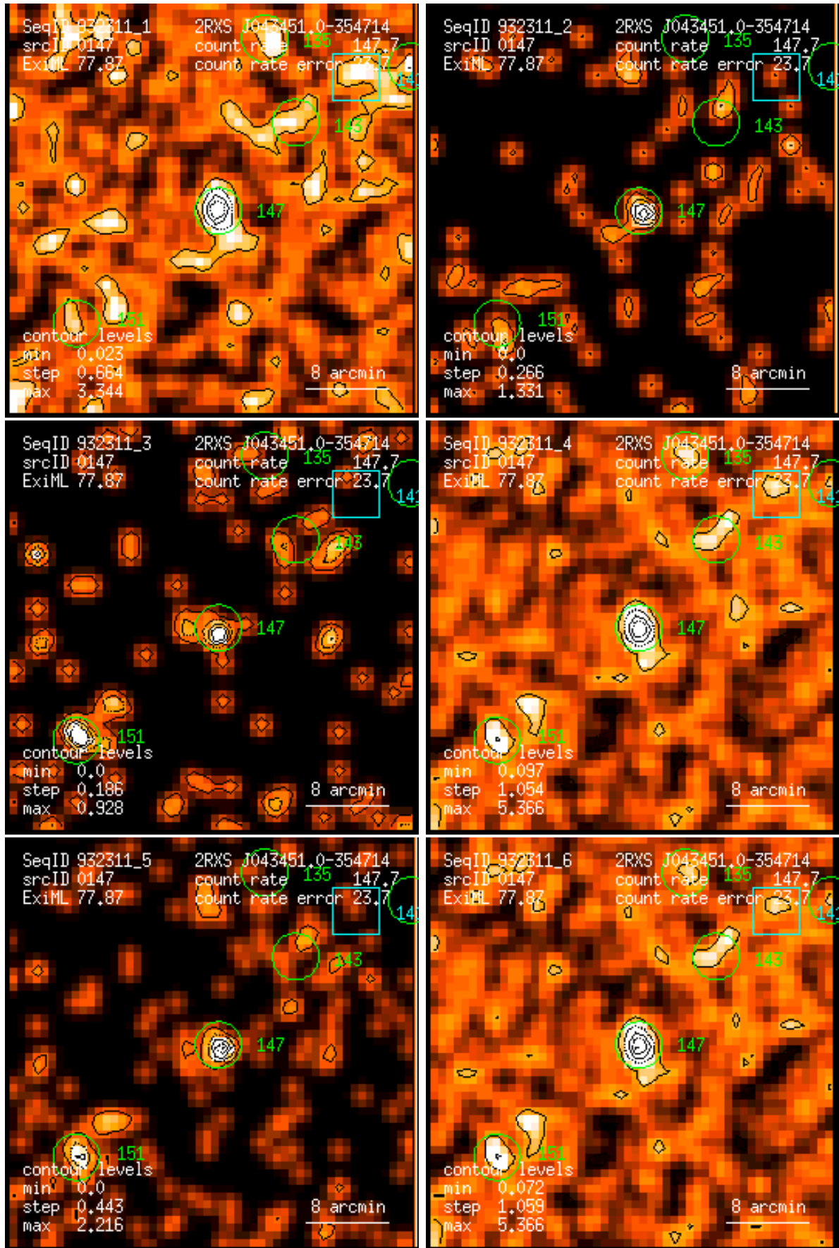
Figure 147: RASS 932311: detection 0147: band rate images, Gaussian filter: (1) PSPC channels 11 – 41, (2) 52 – 90, (3) 91 – 201, (4) 11 – 235, (5) 52 – 201, (6) 11 – 201. Broad band rates in counts/ks. Band rate contour levels in counts/ks/arcmin 2 .
