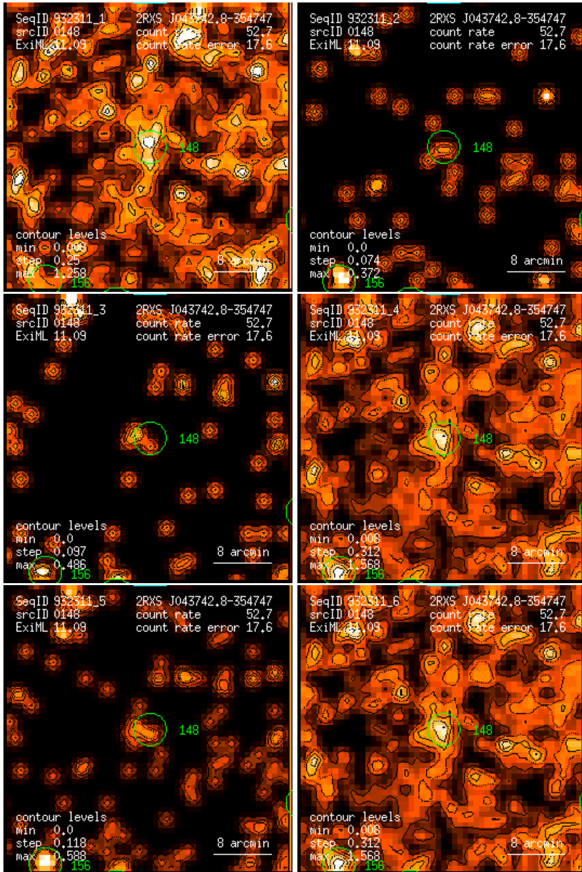
Figure 148: RASS 932311: detection 0148: band rate images, Gaussian filter: (1) PSPC channels 11 – 41, (2) 52 – 90, (3) 91 – 201, (4) 11 – 235, (5) 52 – 201, (6) 11 – 201. Broad band rates in counts/ks. Band rate contour levels in counts/ks/arcmin 2 .
