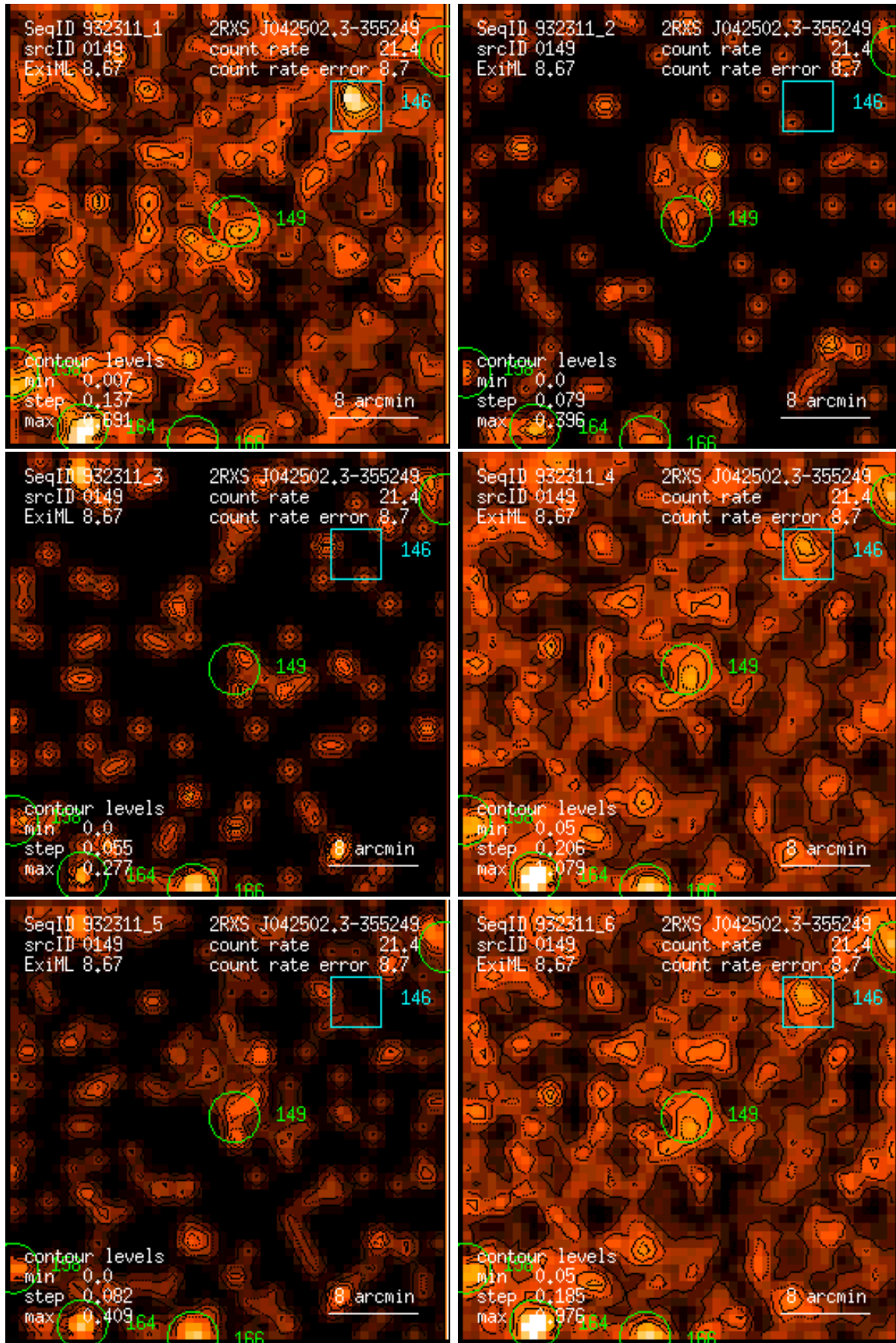
Figure 149: RASS 932311: detection 0149: band rate images, Gaussian filter: (1) PSPC channels 11 – 41, (2) 52 – 90, (3) 91 – 201, (4) 11 – 235, (5) 52 – 201, (6) 11 – 201. Broad band rates in counts/ks. Band rate contour levels in counts/ks/arcmin 2 .
