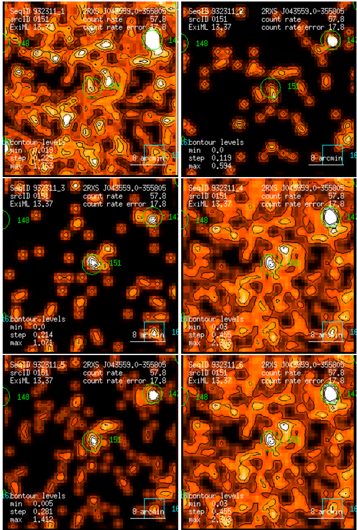
Figure 151: RASS 932311: detection 0151: band rate images, Gaussian filter: (1) PSPC channels 11 – 41, (2) 52 – 90, (3) 91 – 201, (4) 11 – 235, (5) 52 – 201, (6) 11 – 201. Broad band rates in counts/ks. Band rate contour levels in counts/ks/arcmin 2 .
