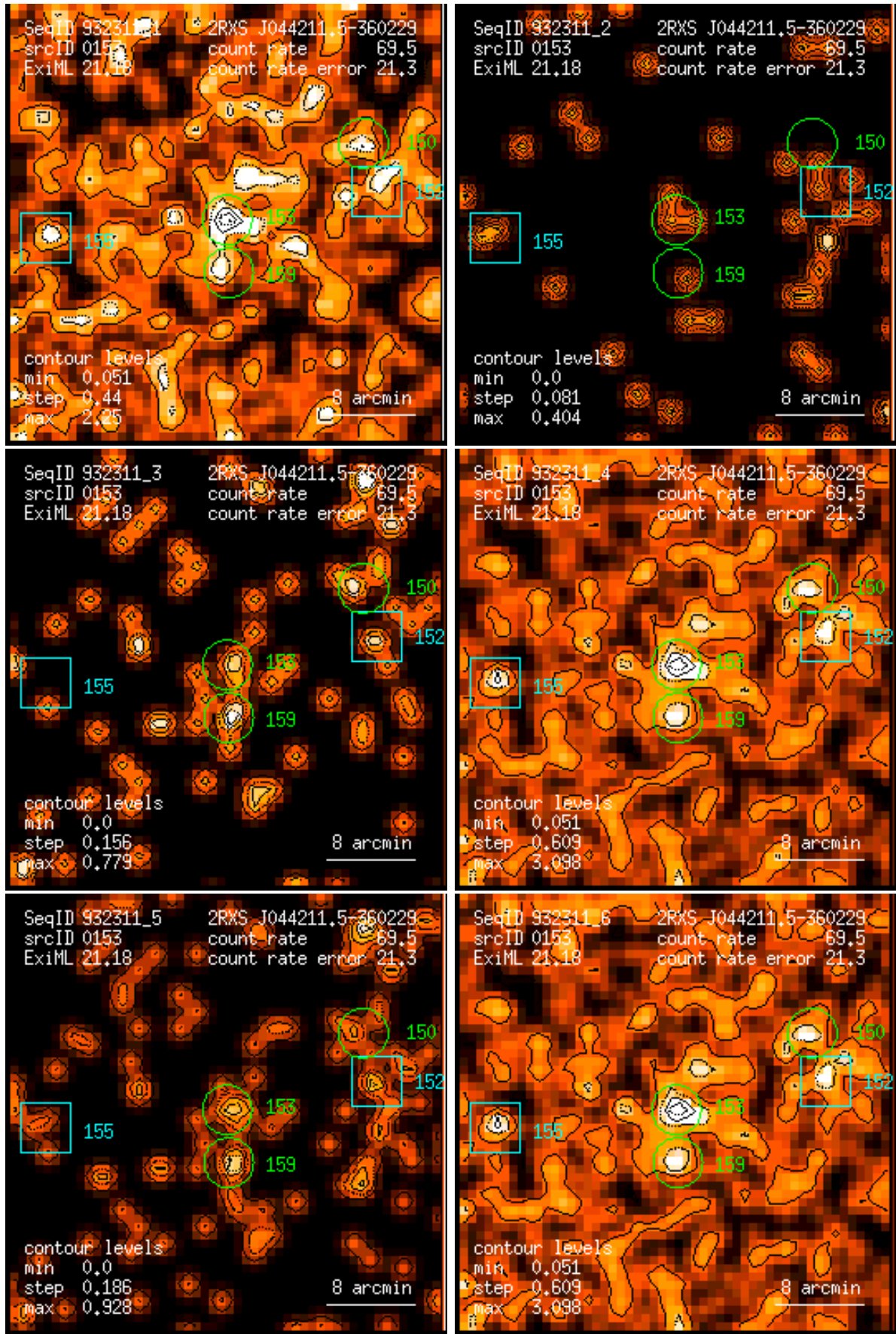
Figure 153: RASS 932311: detection 0153: band rate images, Gaussian filter: (1) PSPC channels 11 – 41, (2) 52 – 90, (3) 91 – 201, (4) 11 – 235, (5) 52 – 201, (6) 11 – 201. Broad band rates in counts/ks. Band rate contour levels in counts/ks/arcmin 2 .
