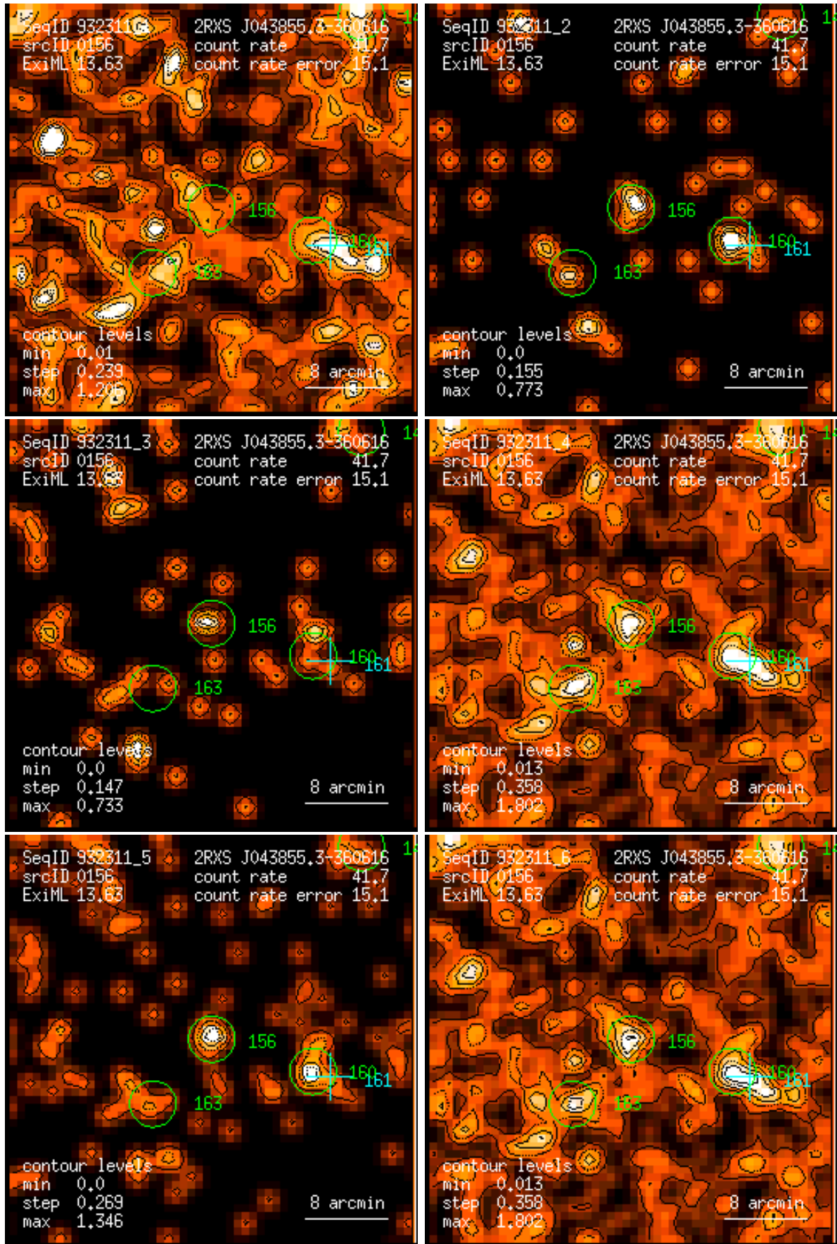
Figure 156: RASS 932311: detection 0156: band rate images, Gaussian filter: (1) PSPC channels 11 – 41, (2) 52 – 90, (3) 91 – 201, (4) 11 – 235, (5) 52 – 201, (6) 11 – 201. Broad band rates in counts/ks. Band rate contour levels in counts/ks/arcmin 2 .
