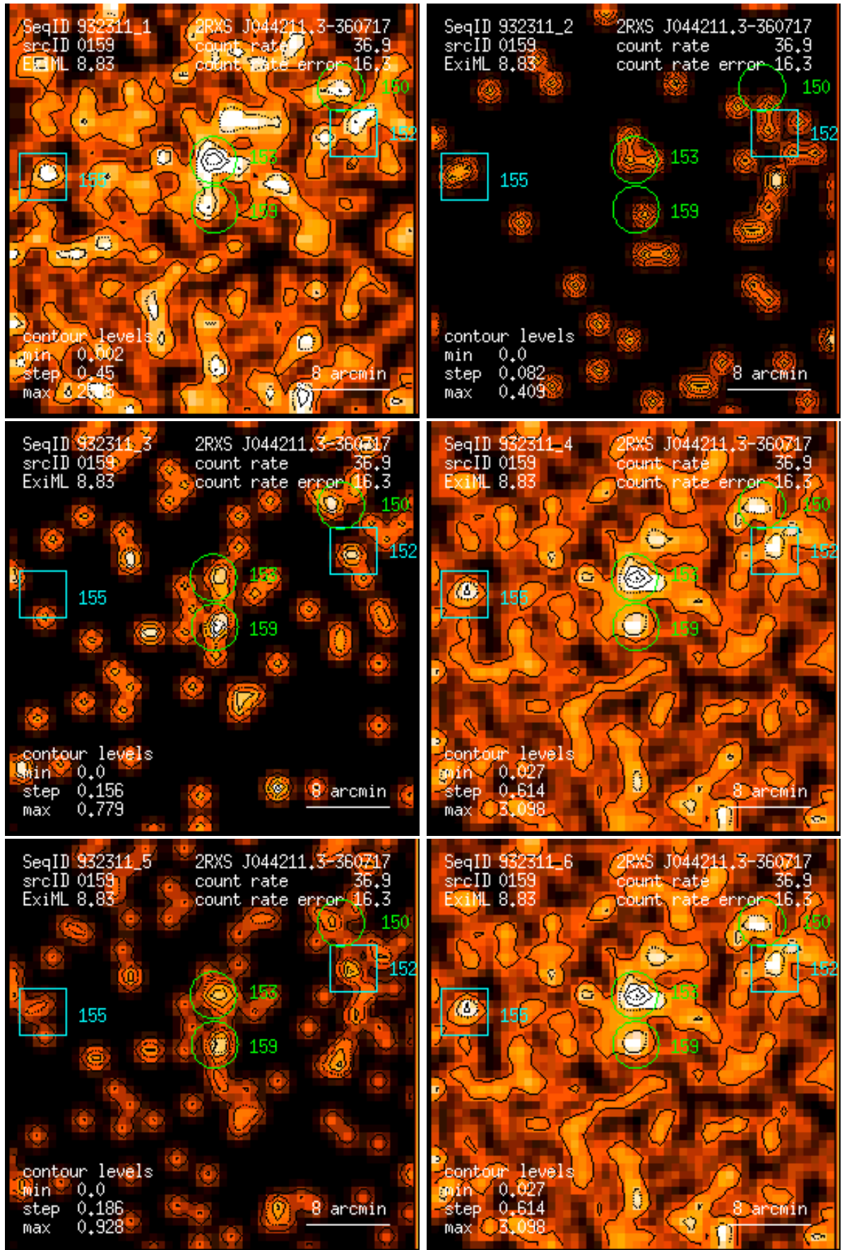
Figure 159: RASS 932311: detection 0159: band rate images, Gaussian filter: (1) PSPC channels 11 – 41, (2) 52 – 90, (3) 91 – 201, (4) 11 – 235, (5) 52 – 201, (6) 11 – 201. Broad band rates in counts/ks. Band rate contour levels in counts/ks/arcmin 2 .
