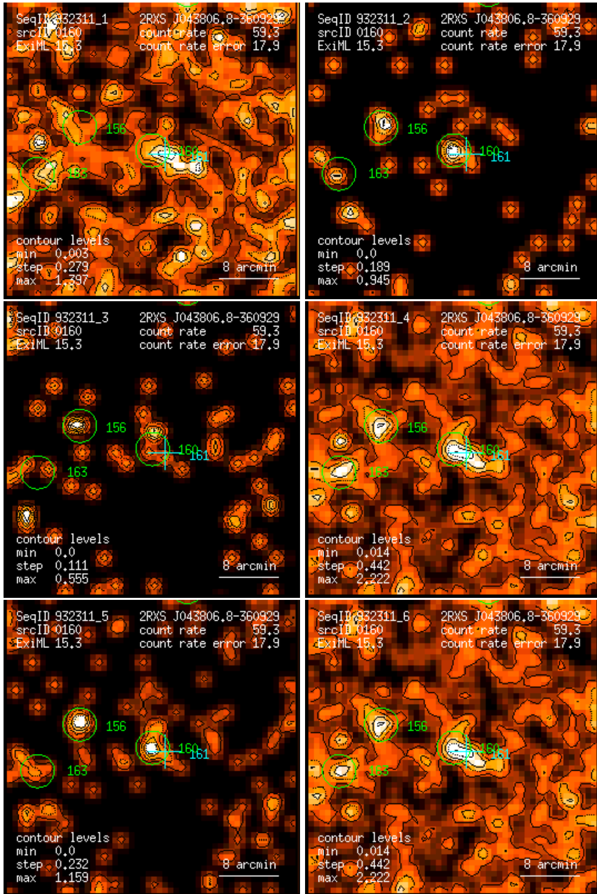
Figure 160: RASS 932311: detection 0160: band rate images, Gaussian filter: (1) PSPC channels 11 – 41, (2) 52 – 90, (3) 91 – 201, (4) 11 – 235, (5) 52 – 201, (6) 11 – 201. Broad band rates in counts/ks. Band rate contour levels in counts/ks/arcmin 2 .
