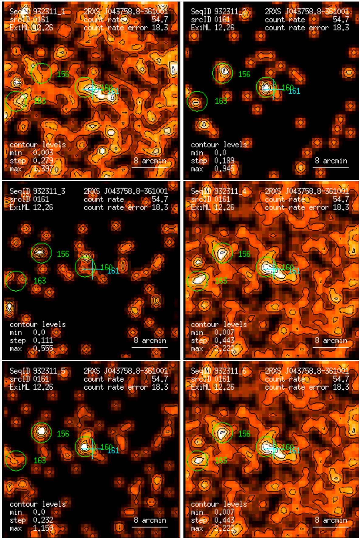
Figure 161: RASS 932311: detection 0161: band rate images, Gaussian filter: (1) PSPC channels 11 – 41, (2) 52 – 90, (3) 91 – 201, (4) 11 – 235, (5) 52 – 201, (6) 11 – 201. Broad band rates in counts/ks. Band rate contour levels in counts/ks/arcmin 2 .
