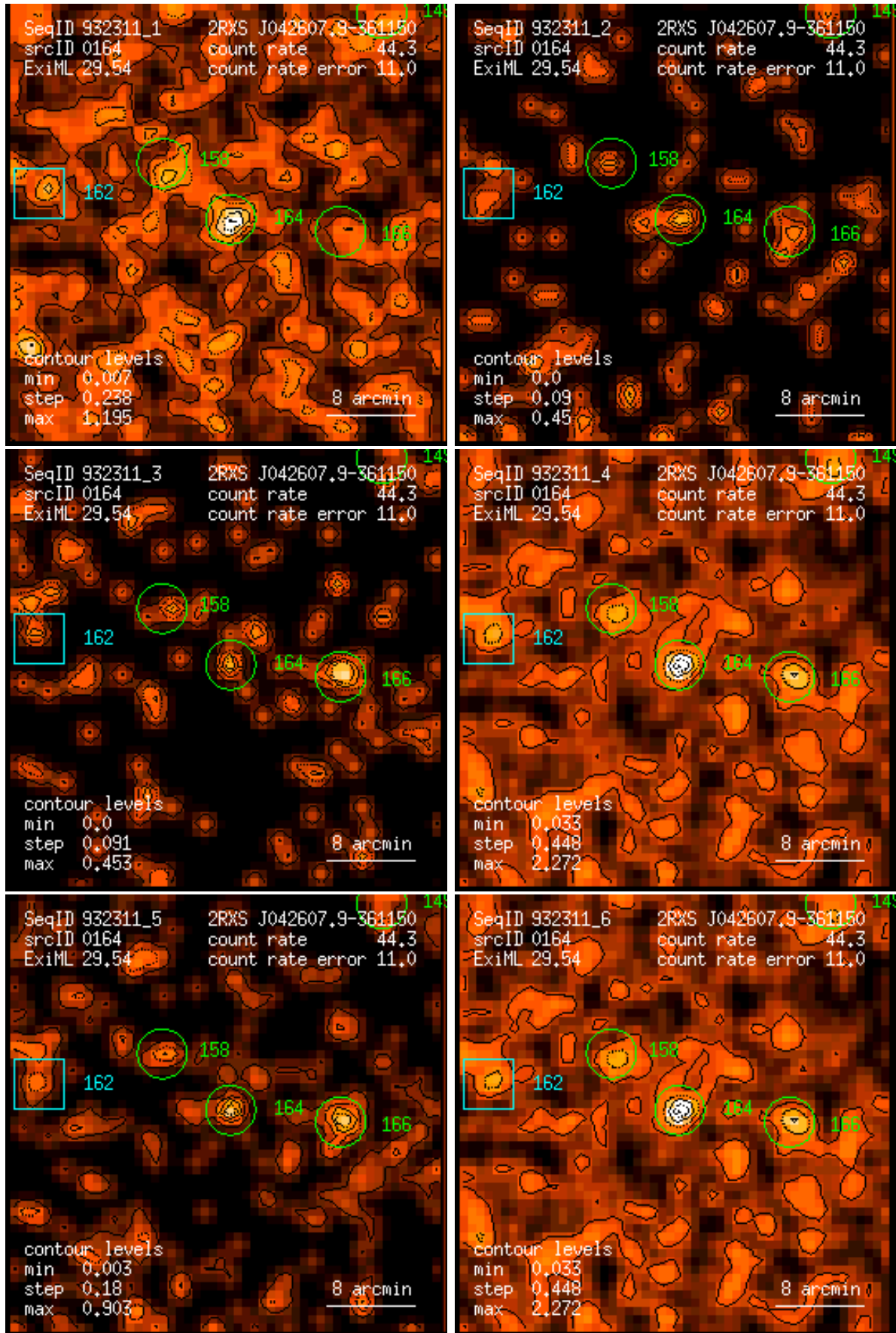
Figure 164: RASS 932311: detection 0164: band rate images, Gaussian filter: (1) PSPC channels 11 – 41, (2) 52 – 90, (3) 91 – 201, (4) 11 – 235, (5) 52 – 201, (6) 11 – 201. Broad band rates in counts/ks. Band rate contour levels in counts/ks/arcmin 2 .
