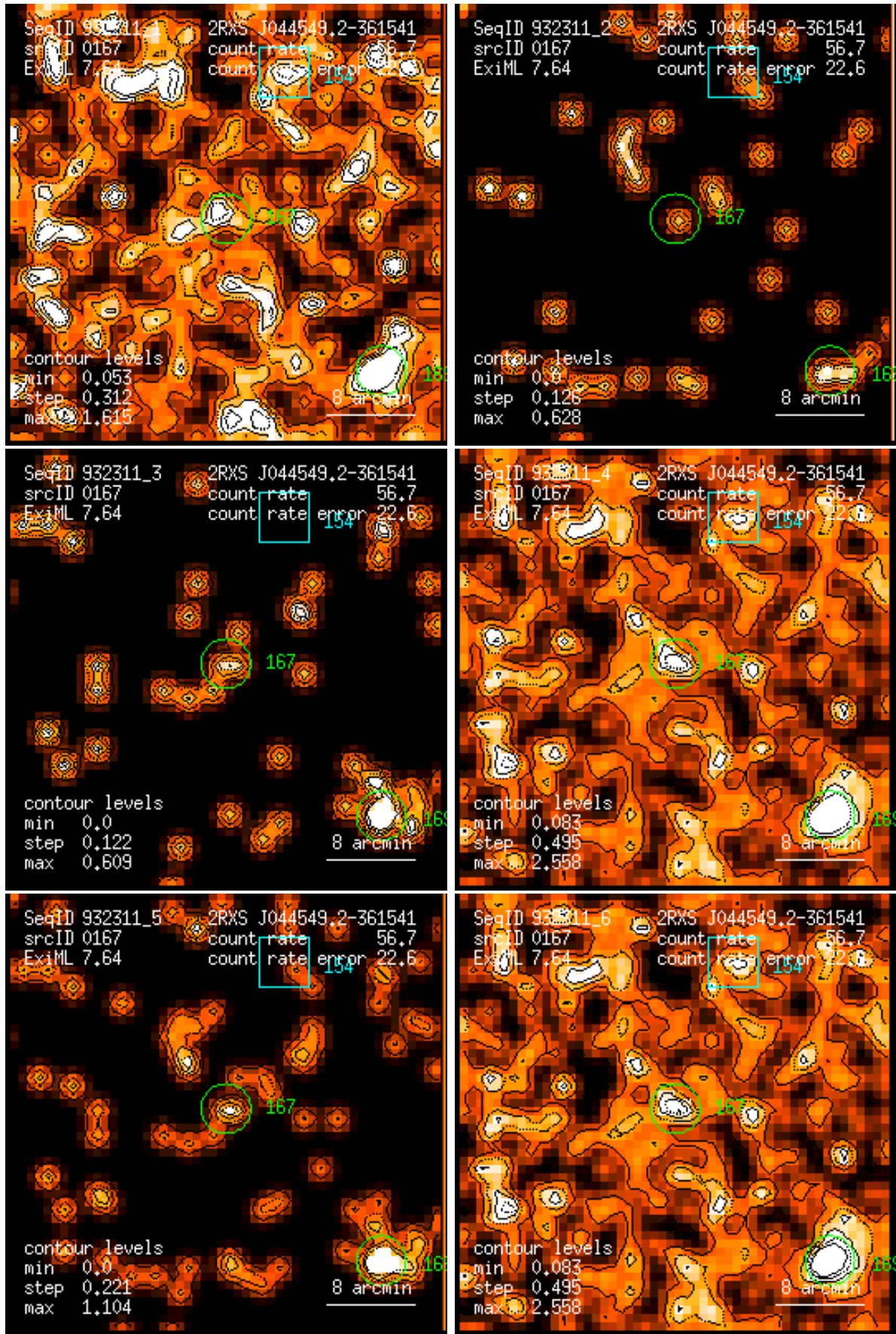
Figure 167: RASS 932311: detection 0167: band rate images, Gaussian filter: (1) PSPC channels 11 – 41, (2) 52 – 90, (3) 91 – 201, (4) 11 – 235, (5) 52 – 201, (6) 11 – 201. Broad band rates in counts/ks. Band rate contour levels in counts/ks/arcmin 2 .
