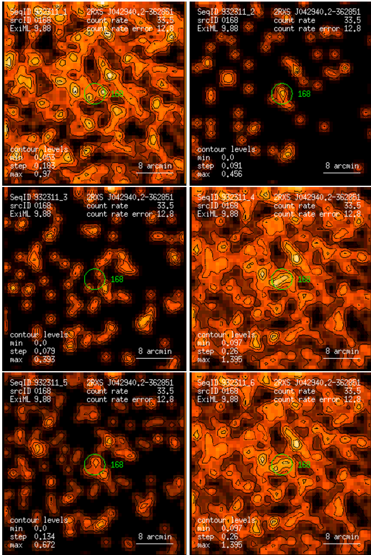
Figure 168: RASS 932311: detection 0168: band rate images, Gaussian filter: (1) PSPC channels 11 – 41, (2) 52 – 90, (3) 91 – 201, (4) 11 – 235, (5) 52 – 201, (6) 11 – 201. Broad band rates in counts/ks. Band rate contour levels in counts/ks/arcmin 2 .
