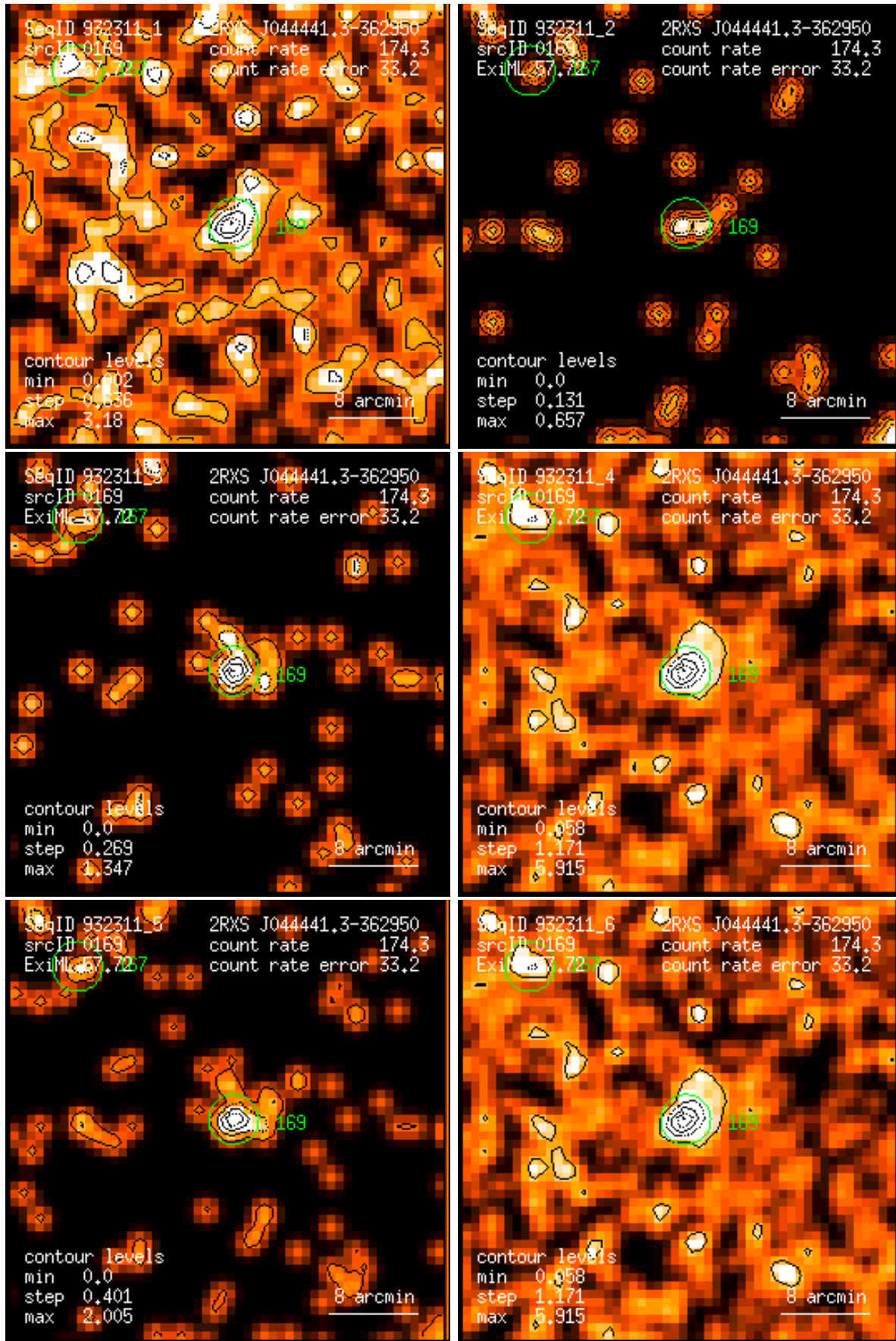
Figure 169: RASS 932311: detection 0169: band rate images, Gaussian filter: (1) PSPC channels 11 – 41, (2) 52 – 90, (3) 91 – 201, (4) 11 – 235, (5) 52 – 201, (6) 11 – 201. Broad band rates in counts/ks. Band rate contour levels in counts/ks/arcmin 2 .
