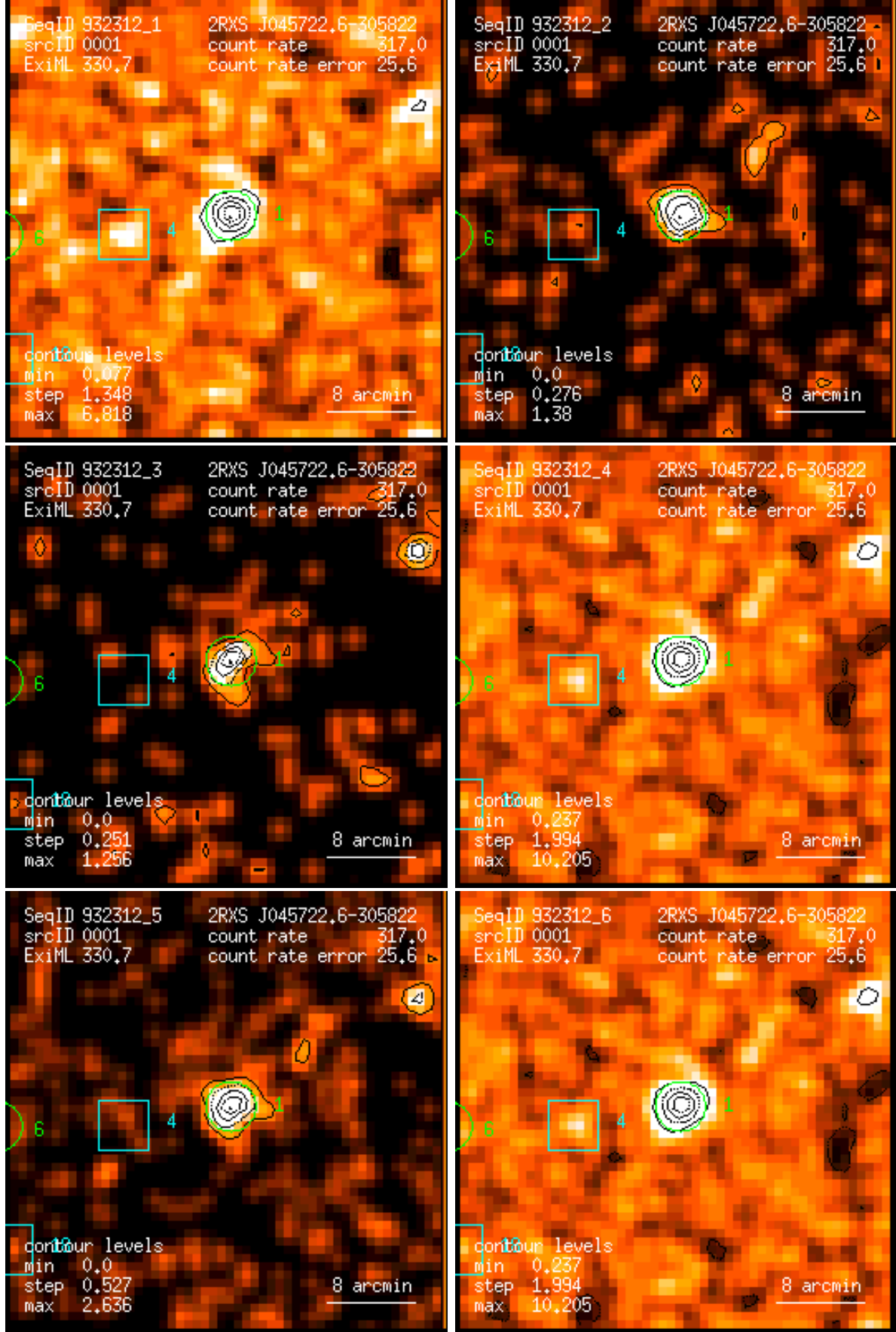
Figure 1: RASS 932312: detection 0001: band rate images, Gaussian filter: (1) PSPC channels 11 – 41, (2) 52 – 90, (3) 91 – 201, (4) 11 – 235, (5) 52 – 201, (6) 11 – 201. Broad band rates in counts/ks. Band rate contour levels in counts/ks/arcmin 2 .
