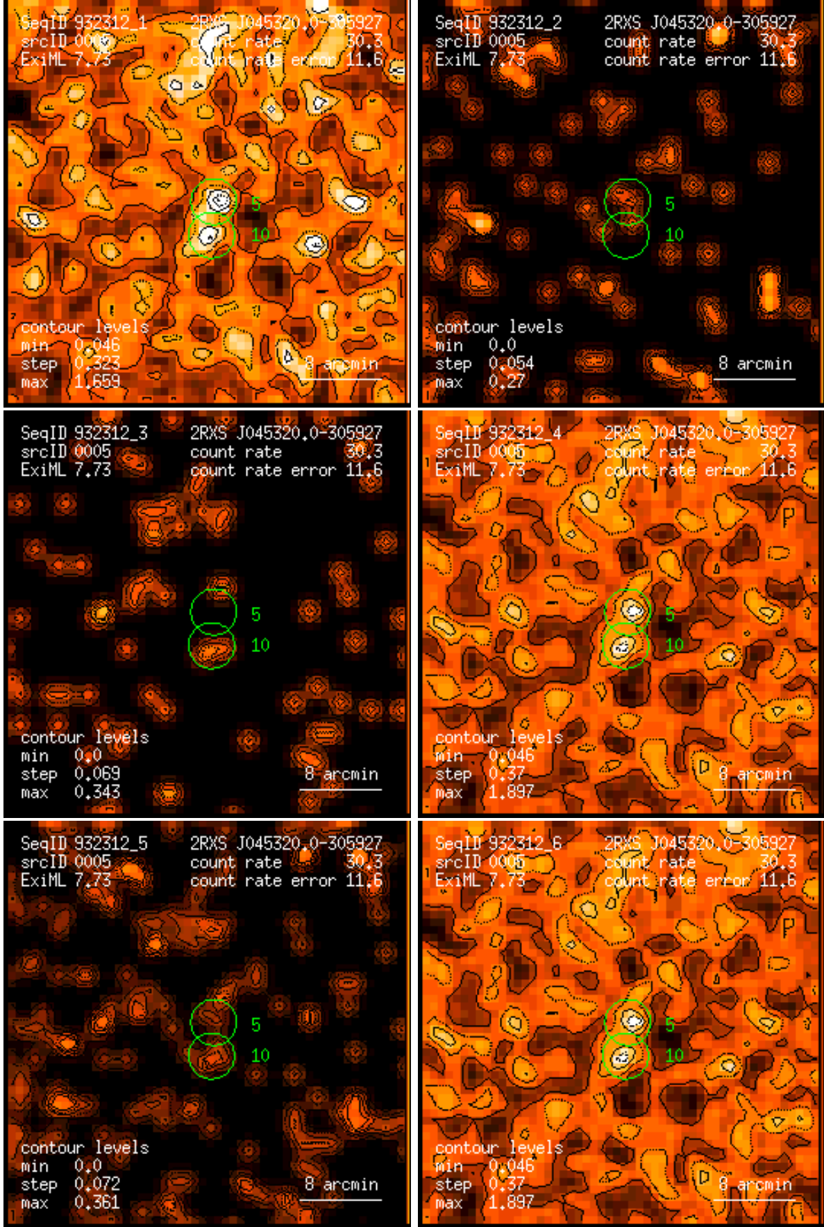
Figure 5: RASS 932312: detection 0005: band rate images, Gaussian filter: (1) PSPC channels 11 – 41, (2) 52 – 90, (3) 91 – 201, (4) 11 – 235, (5) 52 – 201, (6) 11 – 201. Broad band rates in counts/ks. Band rate contour levels in counts/ks/arcmin 2 .
