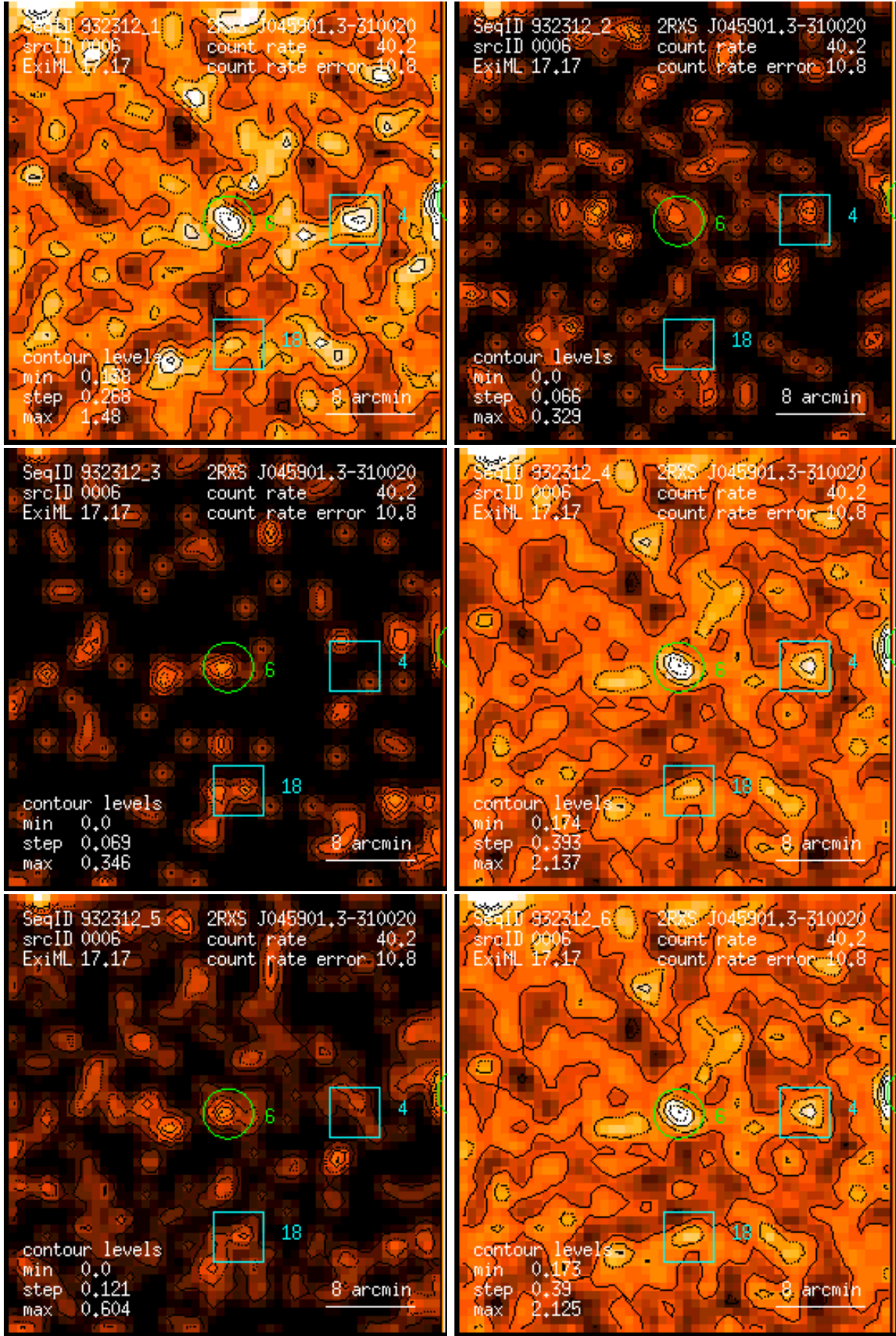
Figure 6: RASS 932312: detection 0006: band rate images, Gaussian filter: (1) PSPC channels 11 – 41, (2) 52 – 90, (3) 91 – 201, (4) 11 – 235, (5) 52 – 201, (6) 11 – 201. Broad band rates in counts/ks. Band rate contour levels in counts/ks/arcmin 2 .
