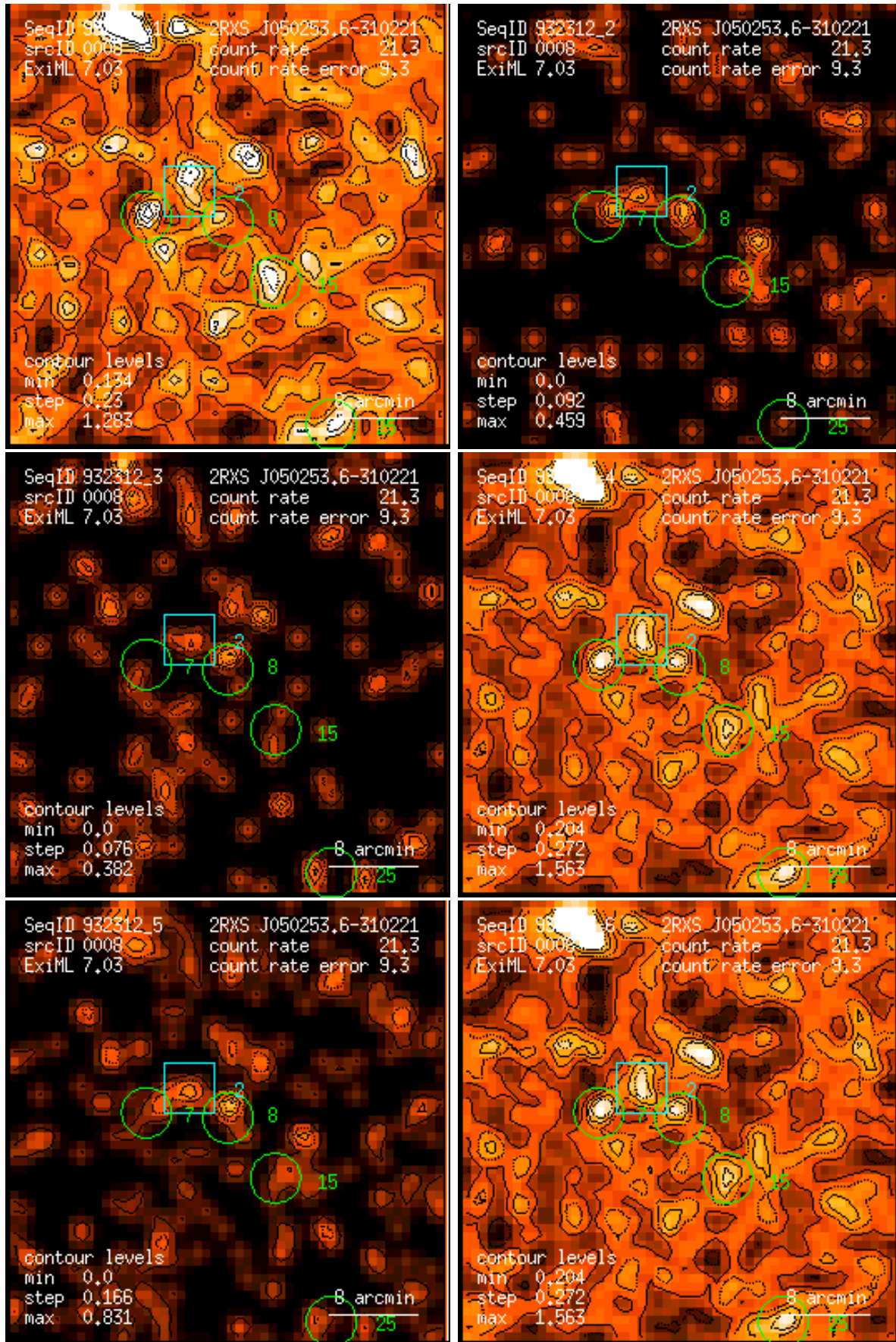
Figure 8: RASS 932312: detection 0008: band rate images, Gaussian filter: (1) PSPC channels 11 – 41, (2) 52 – 90, (3) 91 – 201, (4) 11 – 235, (5) 52 – 201, (6) 11 – 201. Broad band rates in counts/ks. Band rate contour levels in counts/ks/arcmin 2 .
